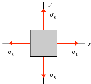
stress element
