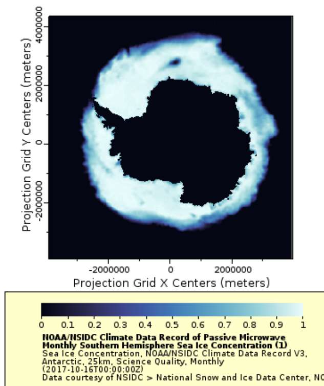
A monthly composite image of Antarctic Sea Ice Concentration showing a polynya, a large ice-free area surrounded by sea ice, in the western Lazarev Sea (for the period September 17-October 16, 2017). Image credit: NOAA.
