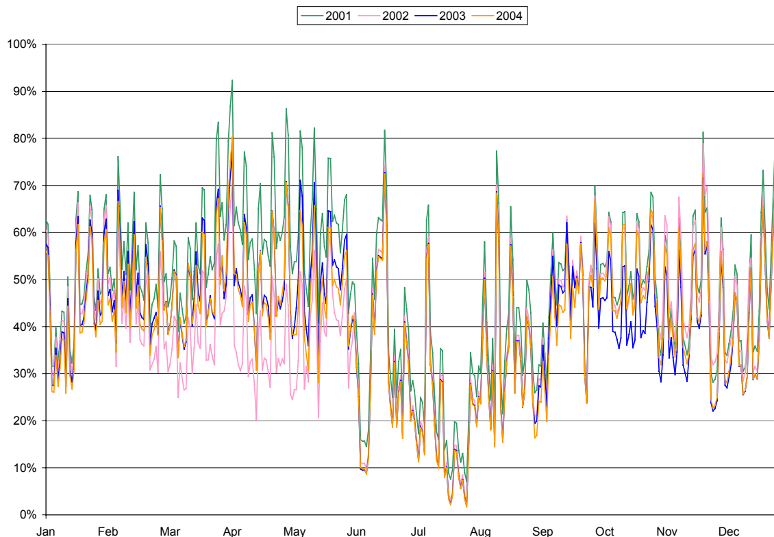
Figure 2. Hourly Reserve Margins for 2001 - 2004
