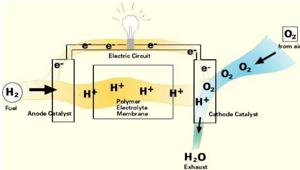
Figure 6-1: Schematic of basic FC operation (Source: [1])
