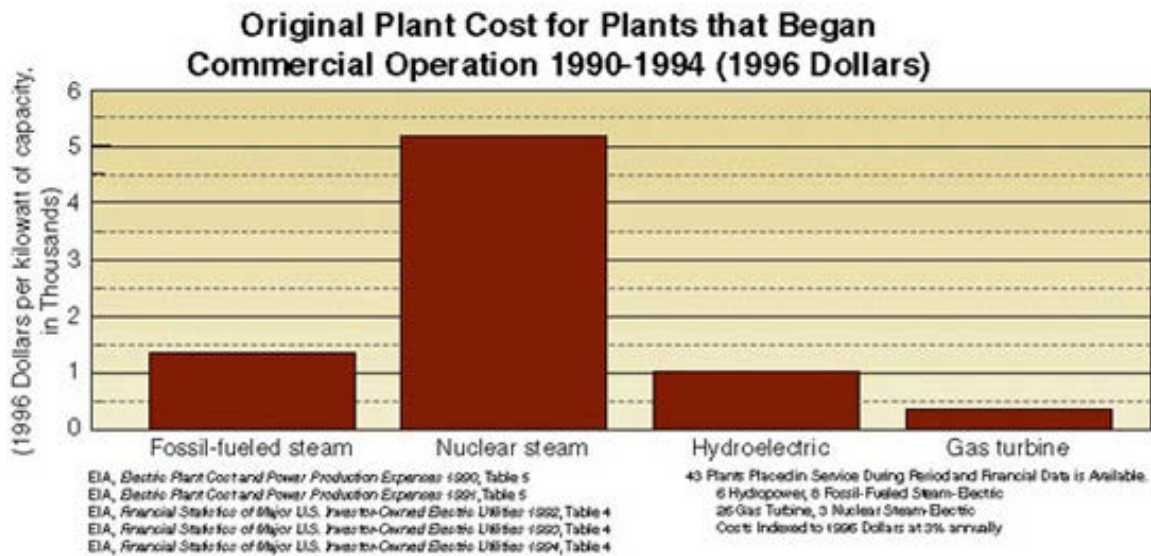
Figure 7-2: Plant costs per unit installed capacity (Source: [2])
