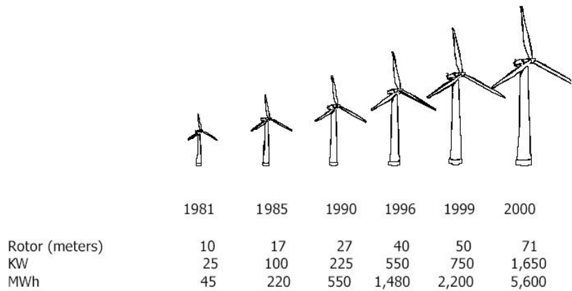
Figure 1-2: Sizes of wind turbines (Source: American Wind Energy Association)
