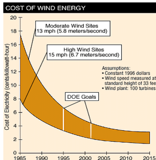
Figure 1-4: Projected cost for wind energy (Source: DOE)
