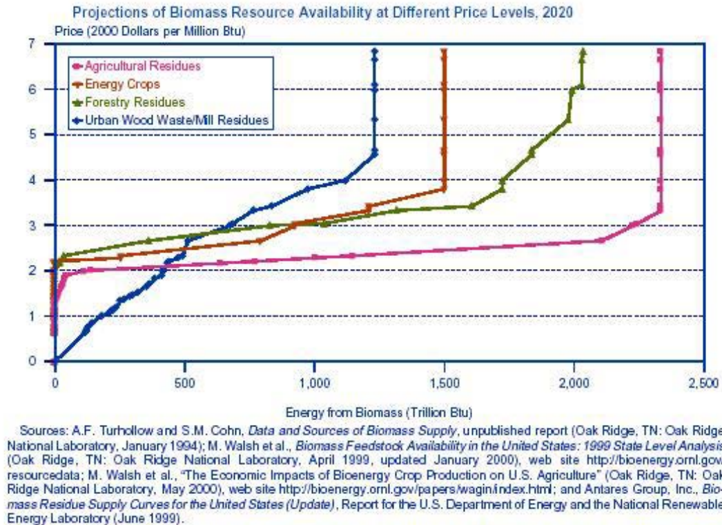
Figure 2-2: POLYSYS estimated biomass supply curve for year 2020 (Source: [4])
