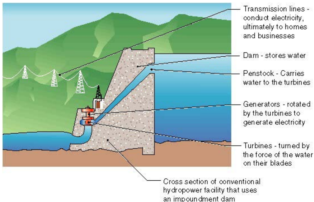
Figure 7-1: Schematic of impoundment hydropower facility (Source: [2])
