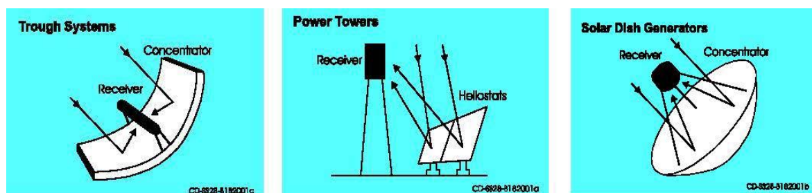
Figure 4-1: Solar-thermal technologies (Source: [2])
