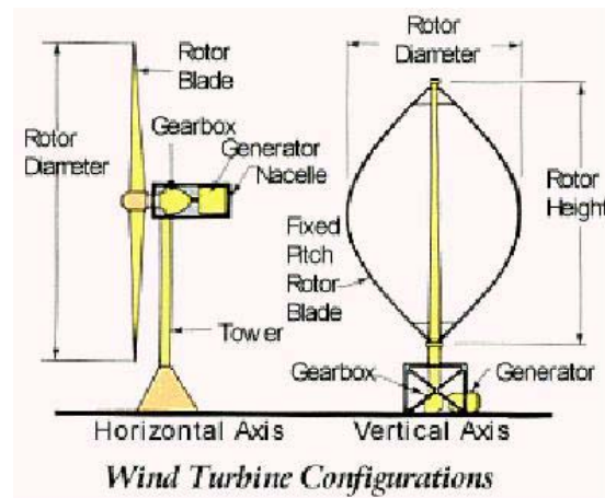
Figure 1-1: Types of wind turbines (Source: American Wind Energy Association)
