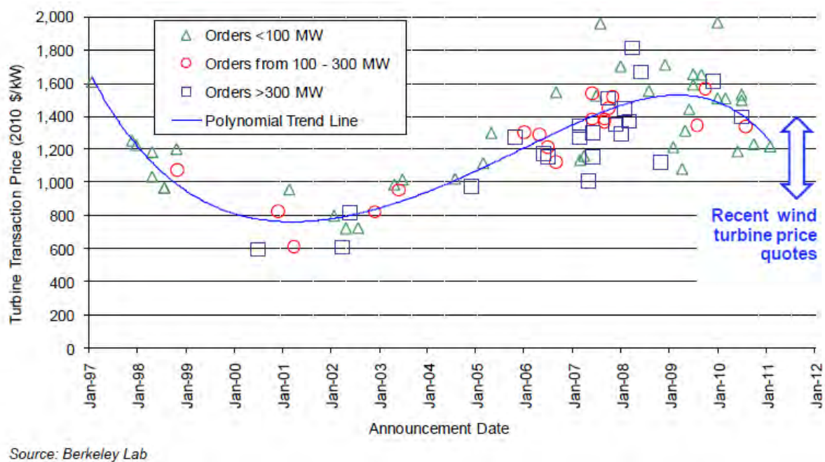
Figure 2-3: Reported U.S. wind turbine prices over time (Source: EERE [6])
