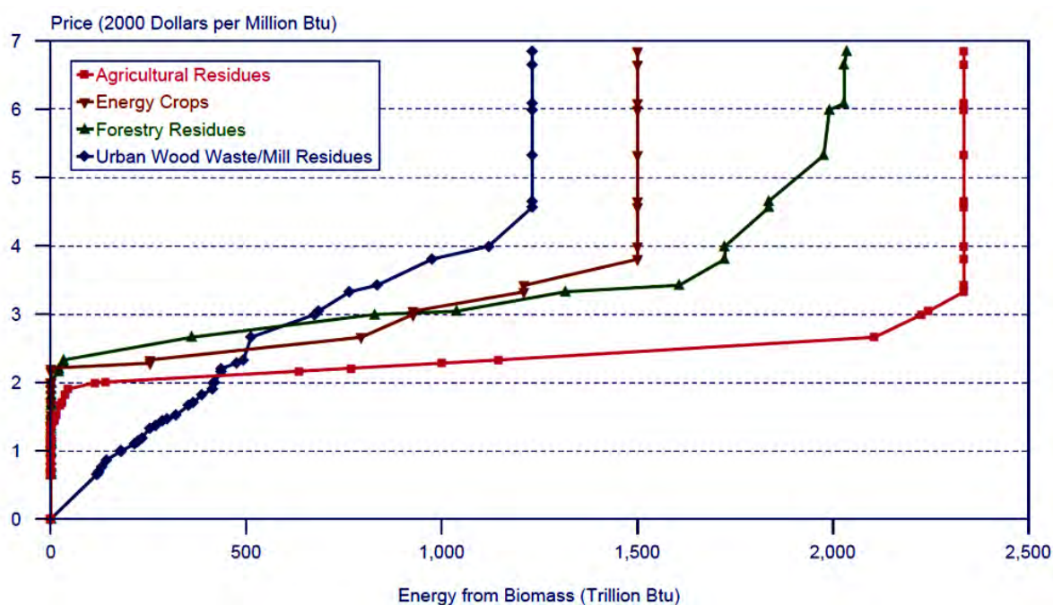
Figure 3-2: POLYSYS estimated biomass supply curve for year 2020 (Source: EIA [11])
