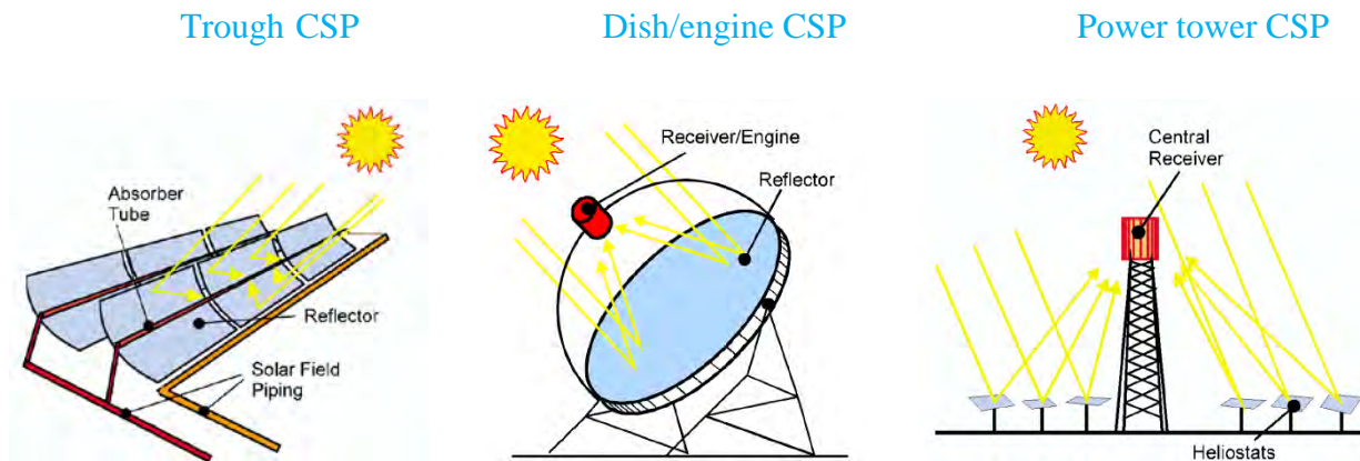
Figure 5-2: Types of concentrating solar power (CSP) collectors (Source: NREL [3])
