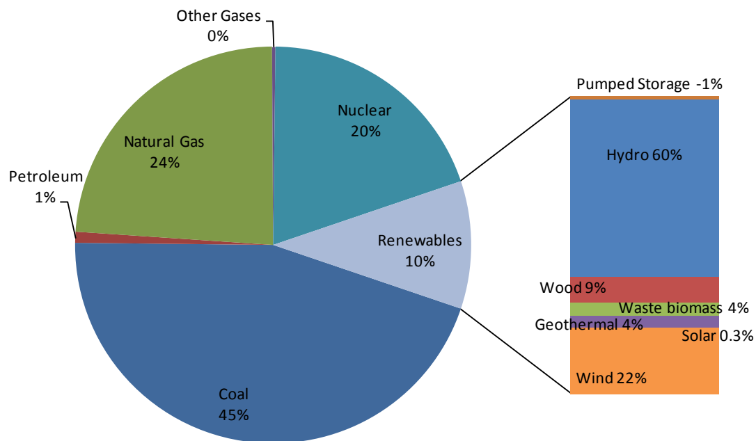
Figure 4-4: Summary of U.S net electricity generation in 2010 (Data source: EIA [13])
