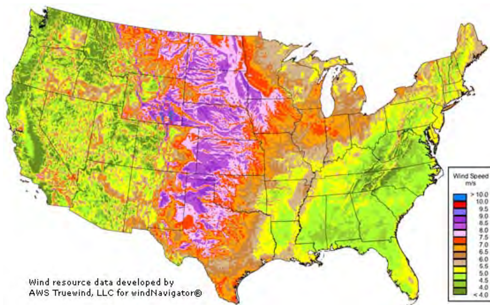
Figure 2-9: 80-meter onshore wind resource map (Source: EERE [8])
