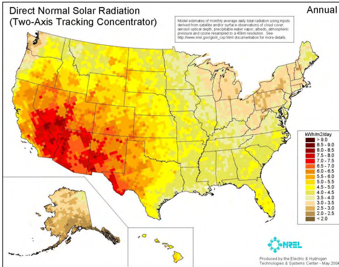
Figure 5-7: Solar resource available to a tracking concentrator (Source: NREL [10])
