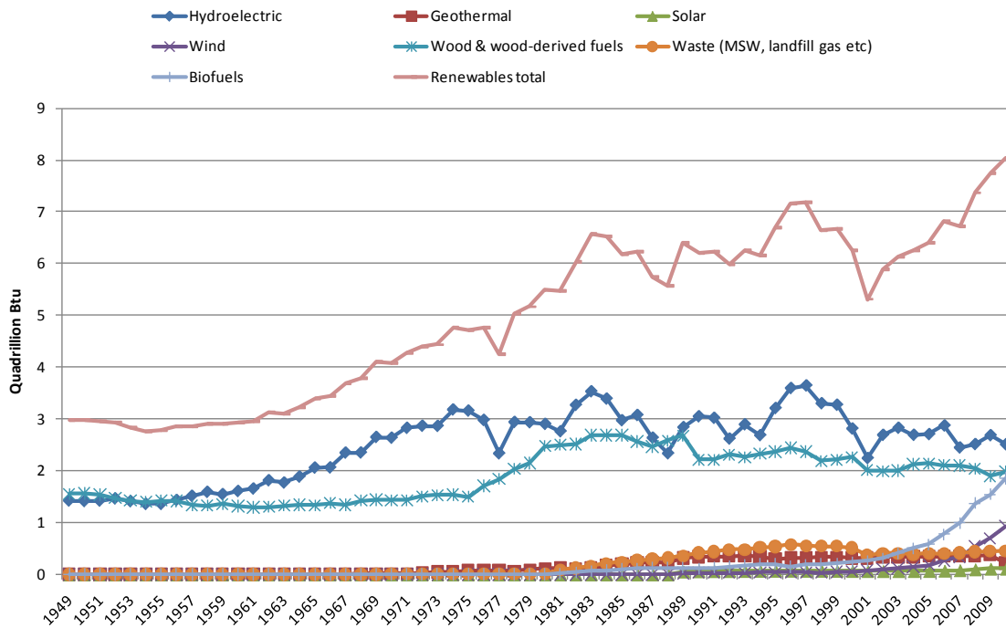
Figure 4-1: U.S. renewable energy consumption 1949-2009 (Source: EIA [1])
