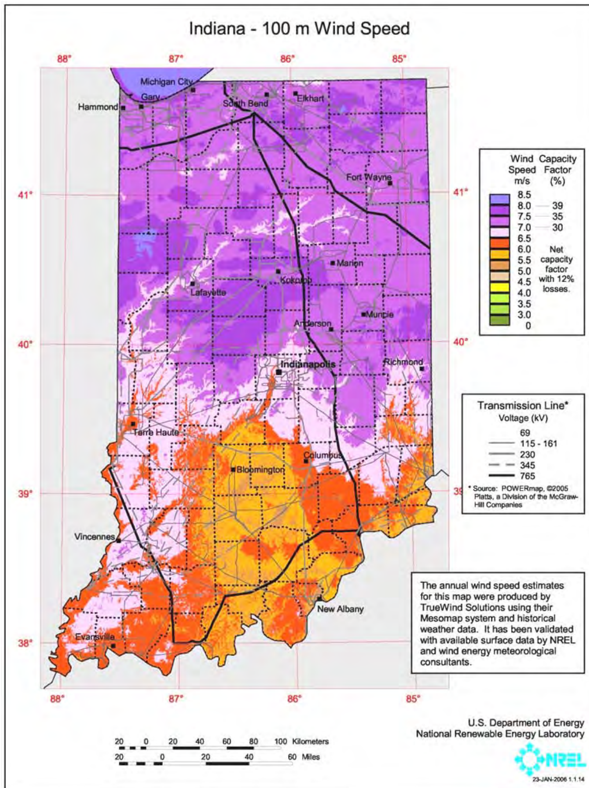
Figure 2-13: Indiana wind speed at 100 meters height (Source: OED/NREL [9])
