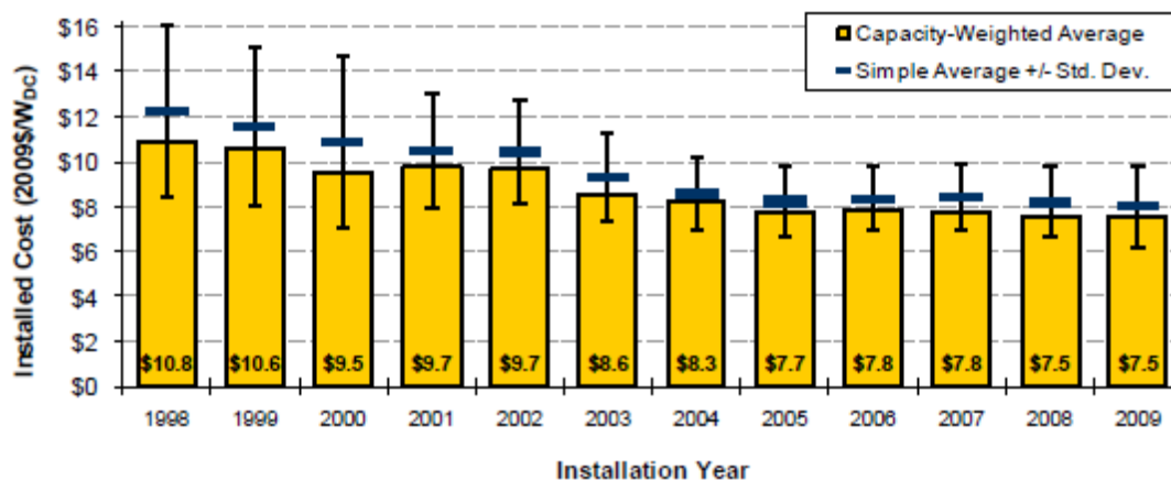
Figure 6-5: Installed cost trends over time (Source: Berkeley [11])
