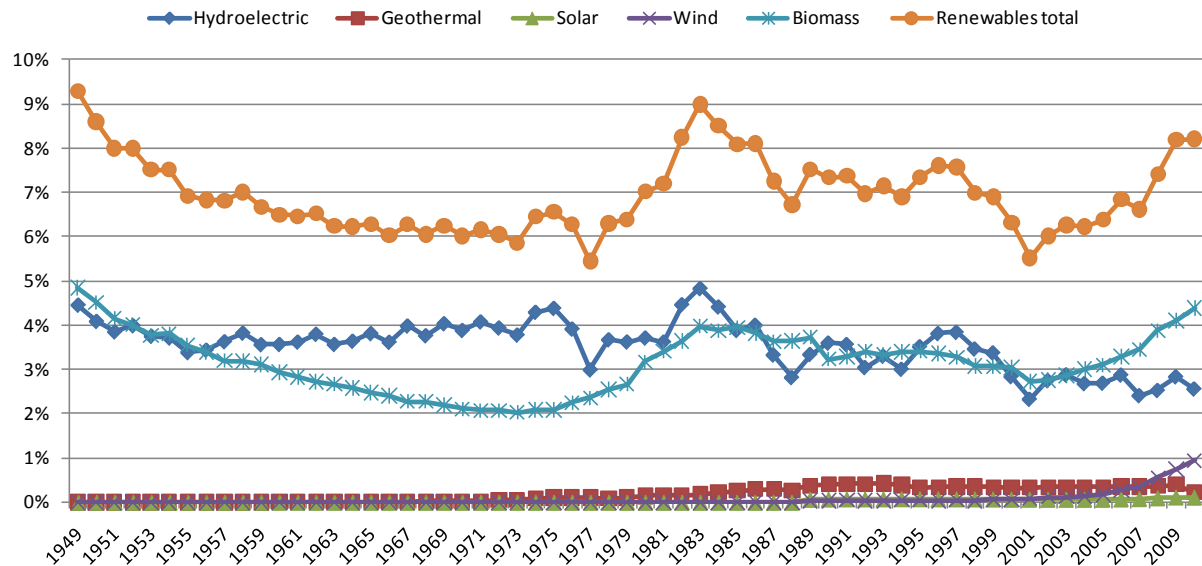
Figure 1-2: U.S. energy consumption by source (1949-2010) (Data source: EIA [1, 2])
