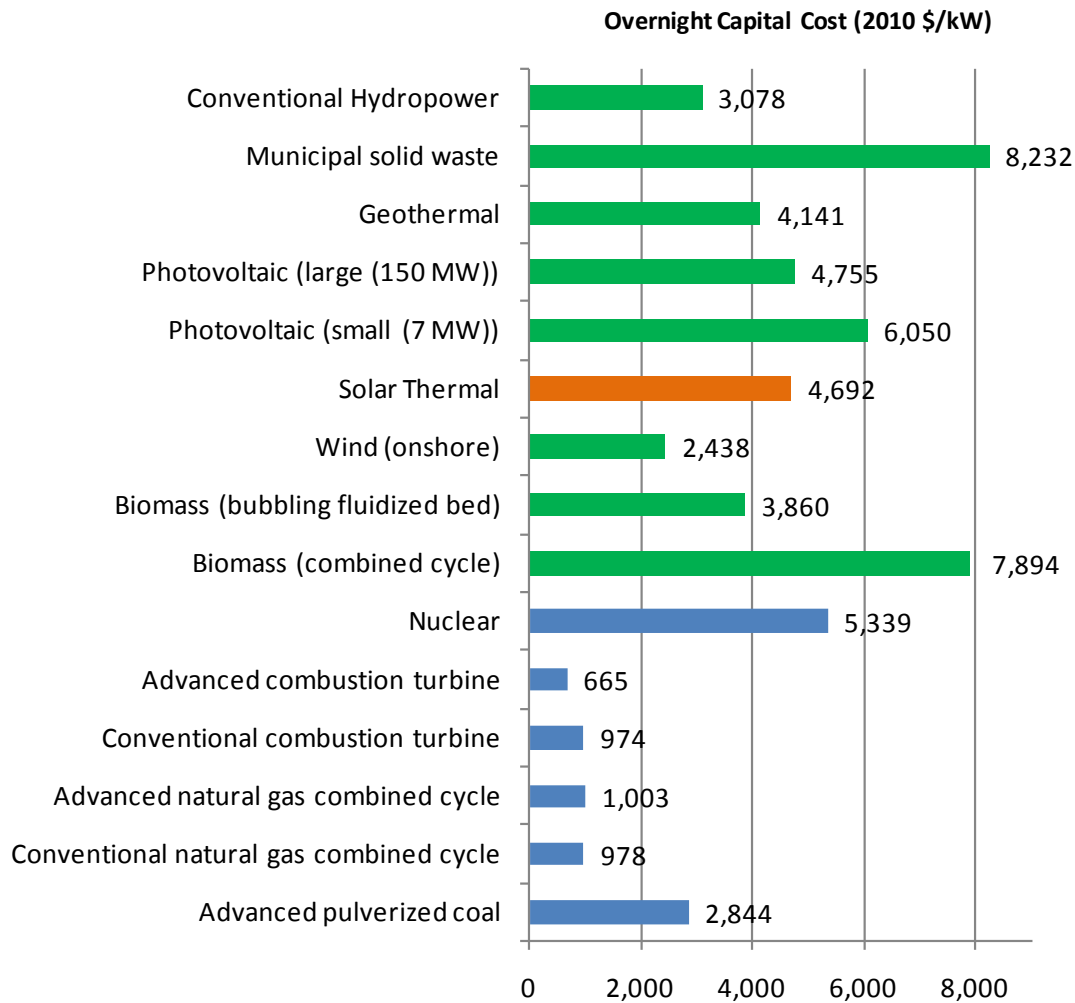
Figure 5-4: Capital cost of generating technologies (Data source: EIA [8])
