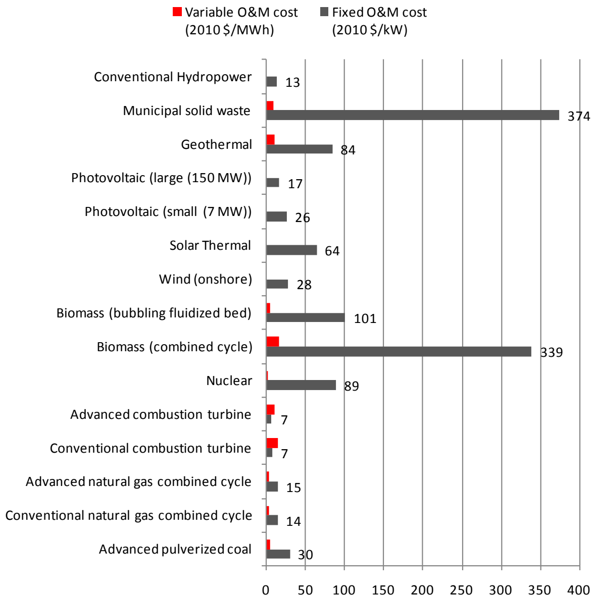
Figure 5-5: Operating and maintenance cost of generating technologies (Data source: EIA [8])
