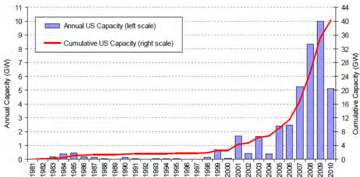
Figure 2-6: Annual capacity additions and cumulative capacity in the U.S. (Source: EERE [6])
