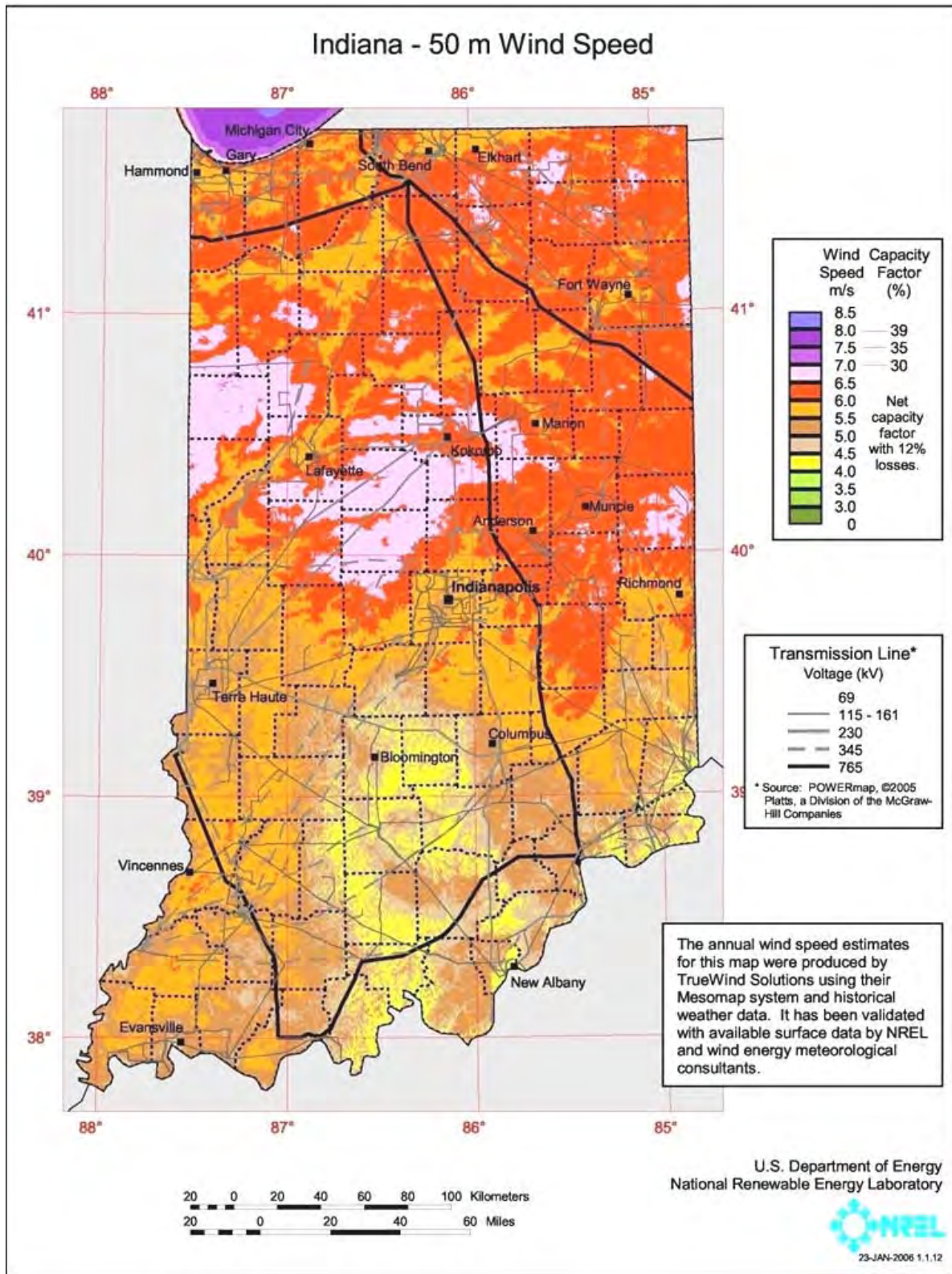
Figure 2-11: Indiana wind speed at 50 meters height (Source: OED/NREL [9])
