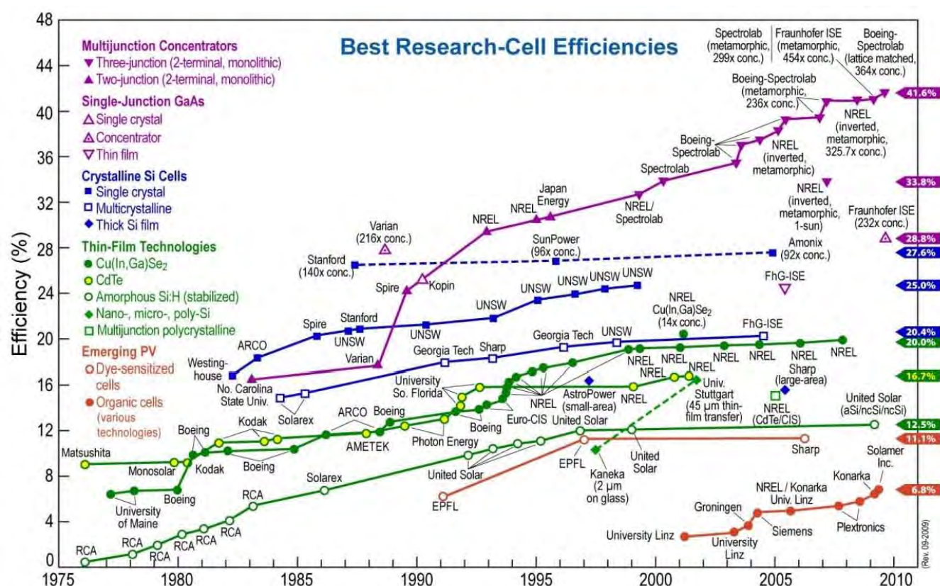
Figure 6-3: Improvements in solar cell efficiency, by system, from 1976 to 2009 (Source: NREL [7])
