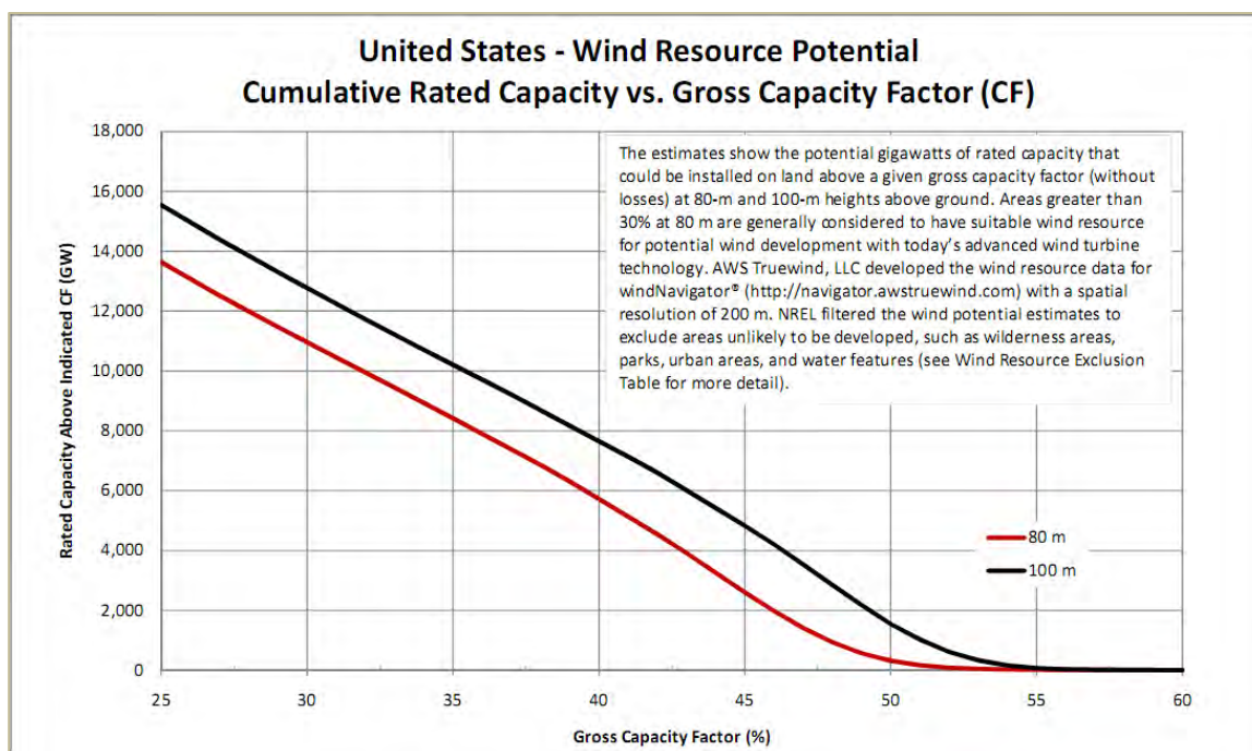
Figure 2-10: U.S. wind resource potential chart (Source: NREL [8])
