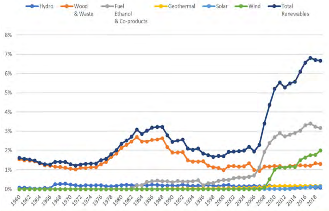
Figure 1-7: Renewables share of Indiana total energy consumption (1960-2019) (Data source: EIA [7])
