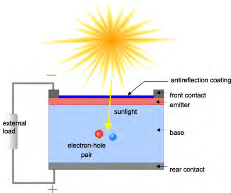
Figure 6-1: Photovoltaic cell operation (Source: EIA [2])
