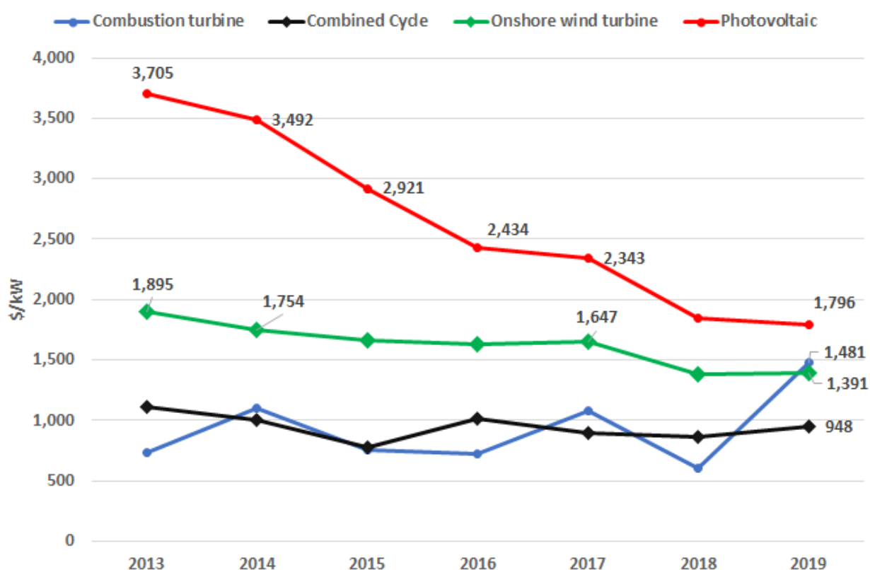
Figure 2-3: Average construction cost of generators installed 2013 to 2019 in the U.S. (Data source: EIA [9, 10])
