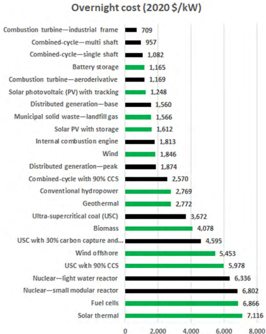
Figure 1-11: Estimated generating technologies capital costs (Data source: EIA [17])
