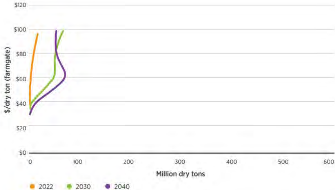
Figure 3-4: Supply curves of potential woody energy crop production for select years under base-case assumptions 10 (Source: DOE [1])
