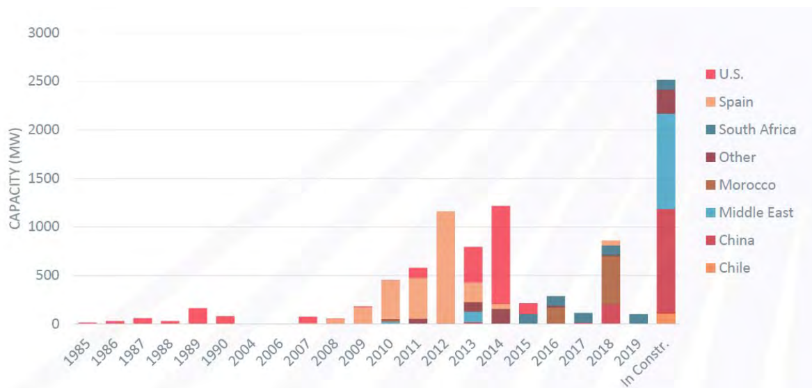
Figure 5-10: Solar thermal power capacity installation worldwide (Sources: U.S. DOE [10])
