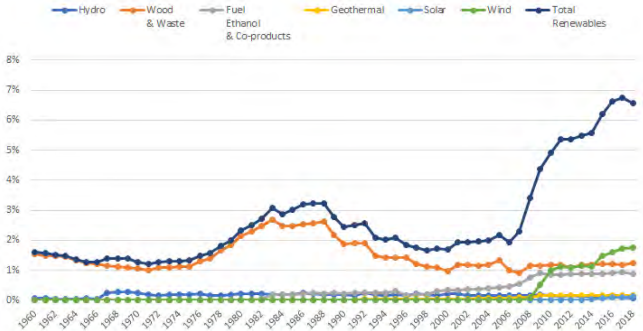
Figure 4-5: Renewables share of Indiana total energy consumption (1960-2018) (Data source EIA [18])
