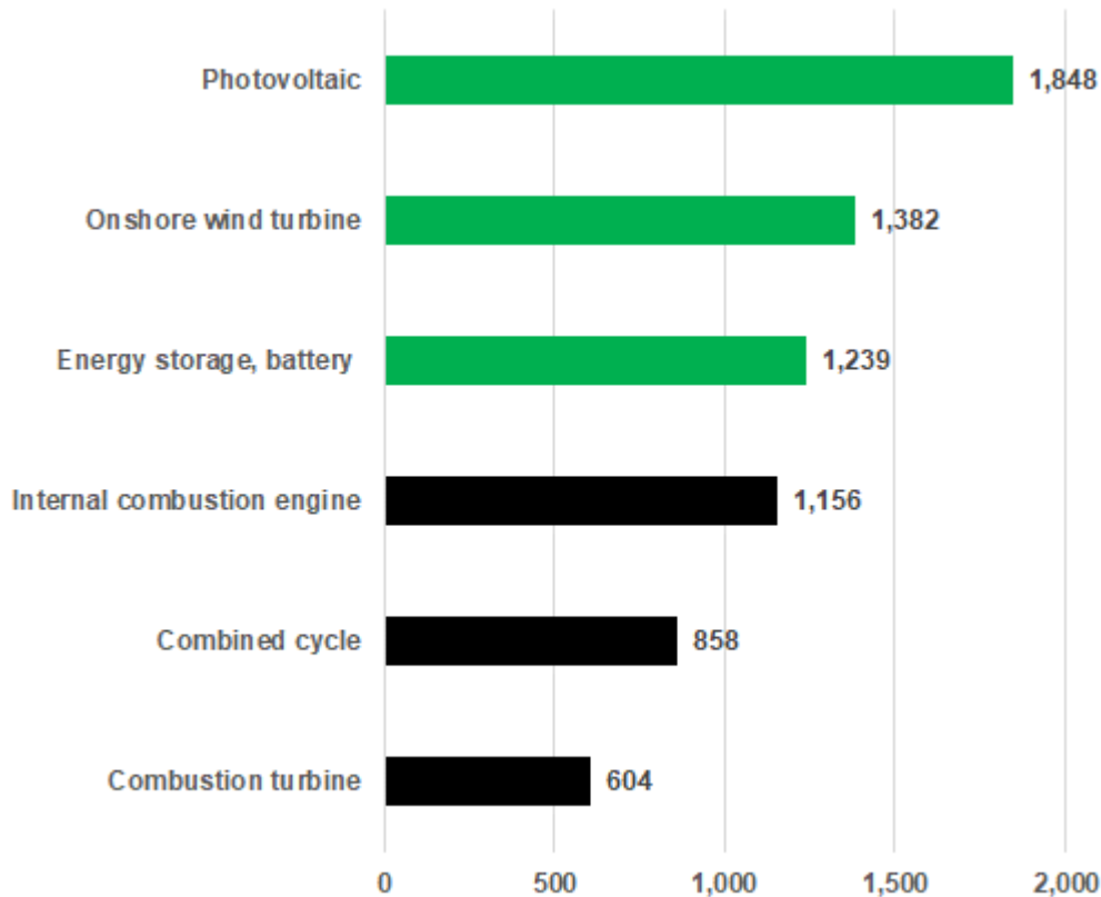
Figure 1-10: Average construction cost ($/kW) of generation installed in 2018 (Data source: EIA [14])
