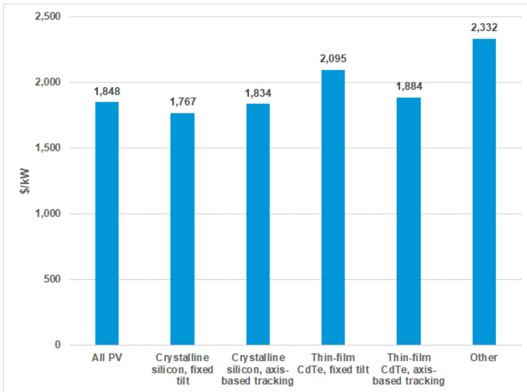
Figure 6-6: Average cost of PV systems of at least 1 MW installed in the U.S. in 2018 (Data Source: EIA [11])
