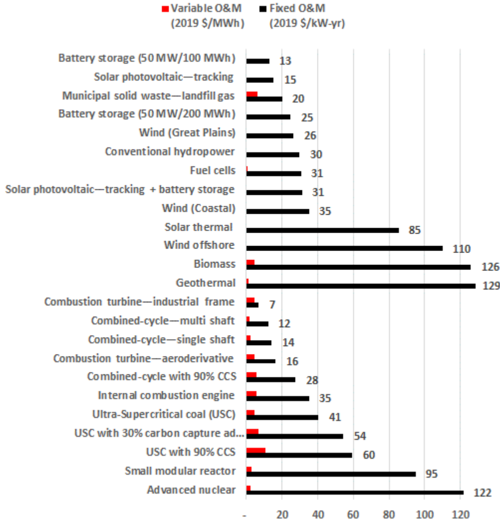
Figure 2-4: Generating technologies O&M costs (Data source: EIA [9])
