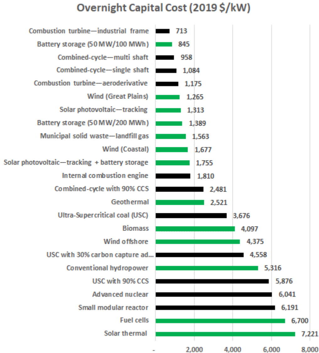
Figure 1-11: Estimated generating technologies capital cost (Data source: EIA [15])
