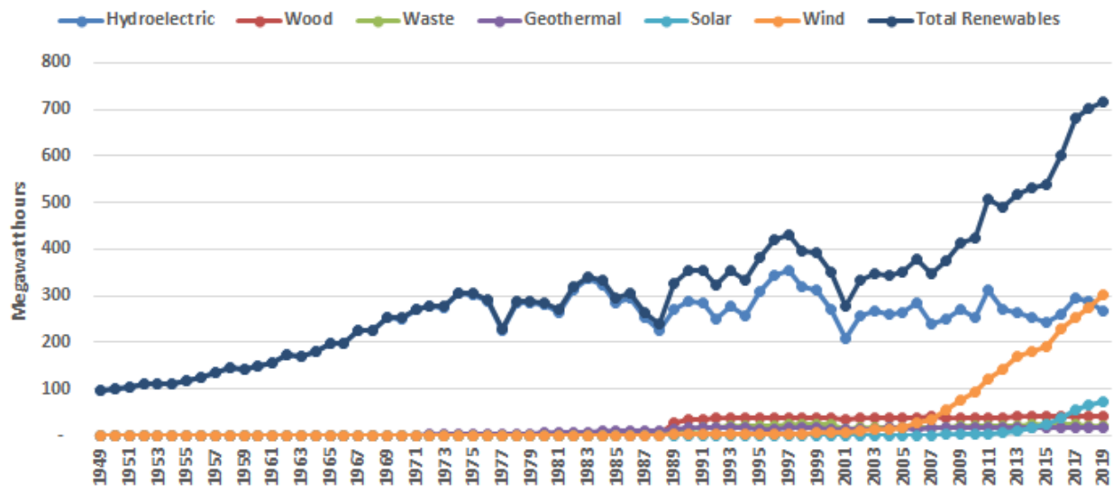
Figure 1-4: Renewable electricity generation in the U.S. (1949-2019) (Data source: EIA [6])
