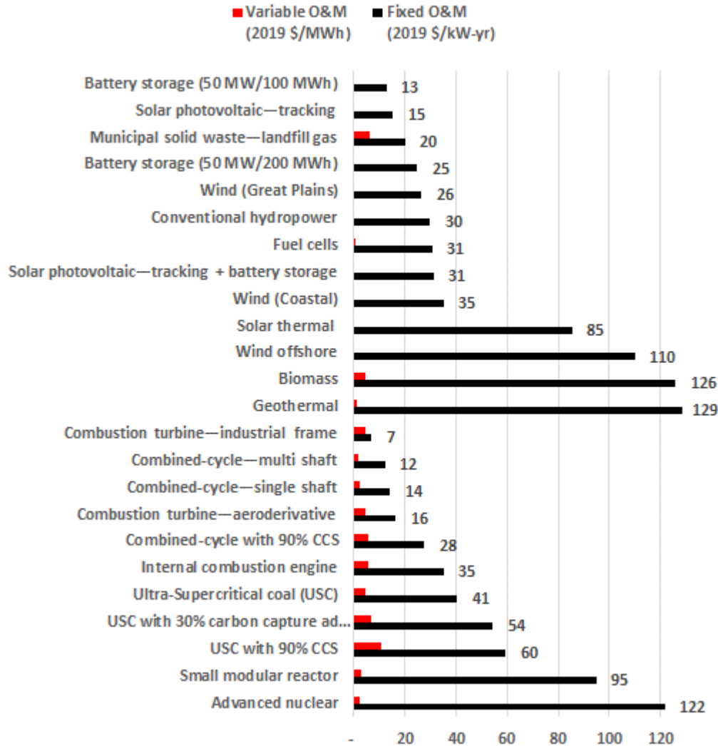
Figure 6-8: Estimated fixed and variable O&M cost of generating technologies (Data source: EIA [12])
