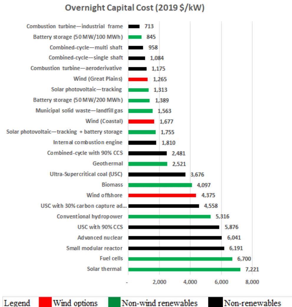
Figure 2-2: Estimated capital costs of various electric generation options (Data source: EIA [9])
