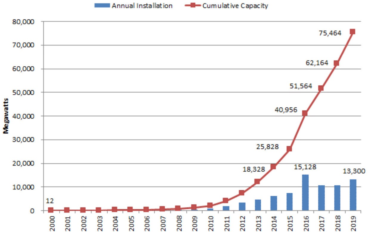
Figure 6-9: Grid-connected U.S. PV installed 2000 to 2018 (Data source: SEIA [4, 13 – 15])
