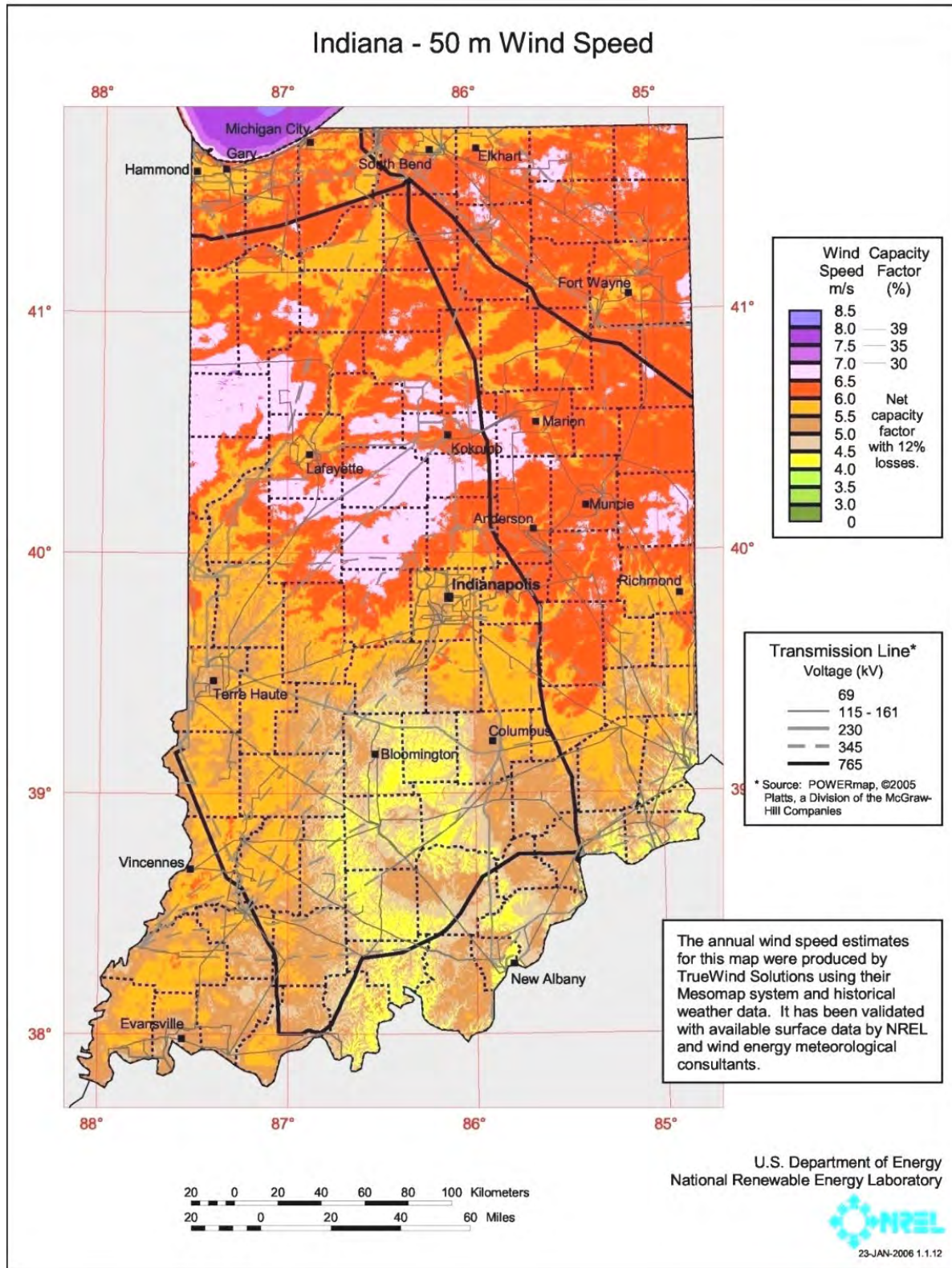
Figure 2-13: Indiana wind speed at 50 meters height (Source: OED/NREL [26])
