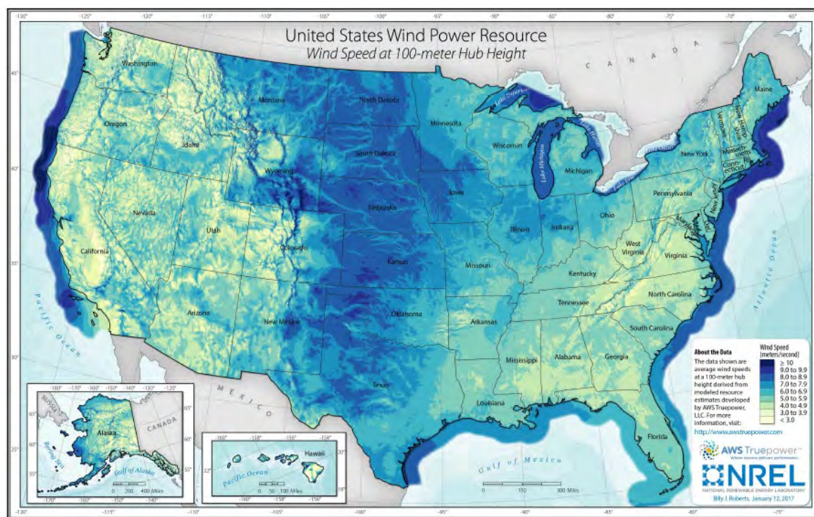
Figure 2-10: 100-meter U.S. wind resource map (Source: DOE [18])
