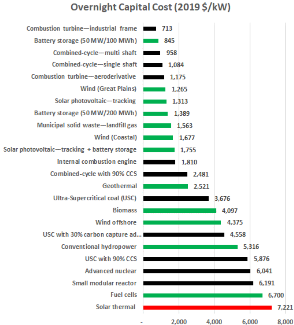
Figure 5-6: Estimated capital cost of generating technologies (Data source: EIA [6])
