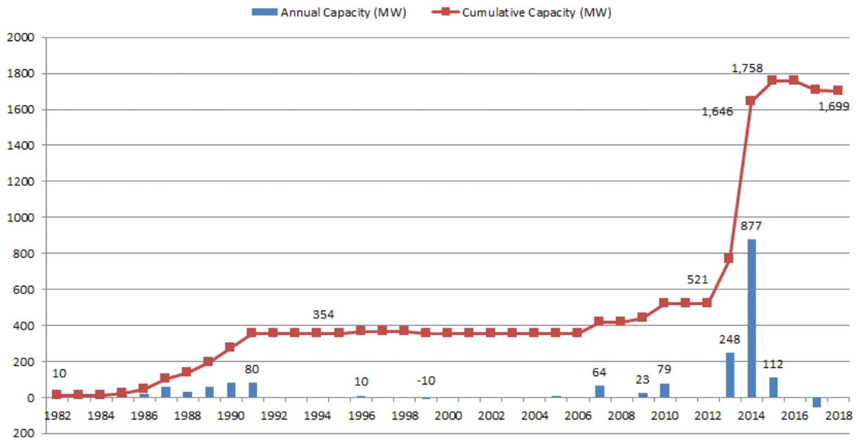
Figure 5-9: Solar thermal power capacity installed in the U.S. (Data sources: NREL [5], SEIA [8], IREC [9])
