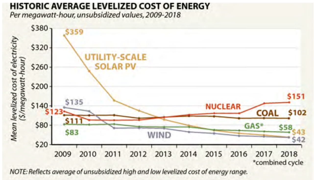
Figure 1-13: Historic average levelized cost of energy from various technologies (Source InsideClimateNews using data from Lazard [16])
