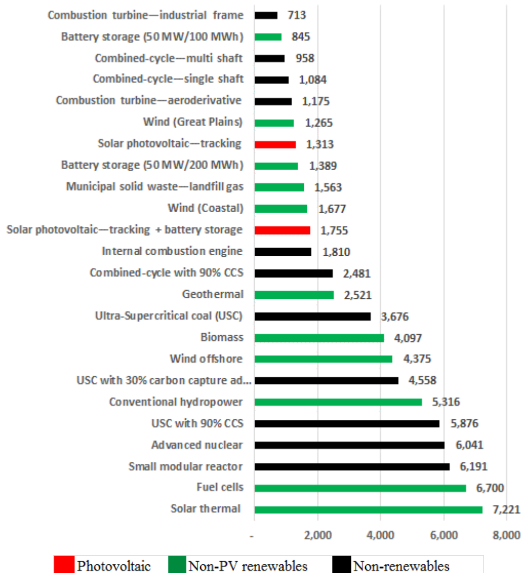
Figure 6-7: Estimated capital cost of generating technologies (Data source: EIA [12])
