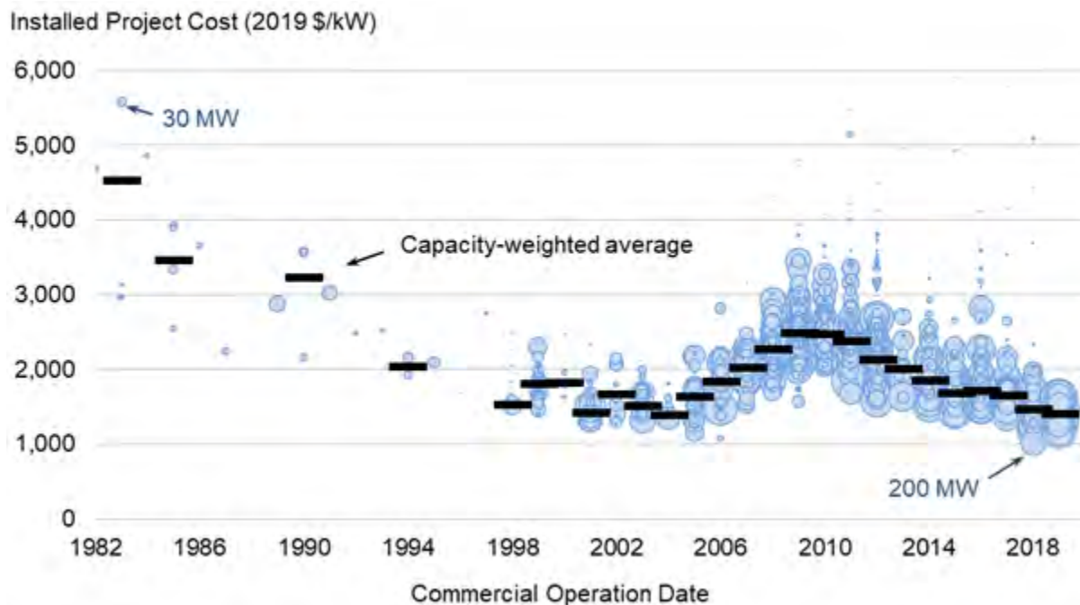
Figure 2-3: Installed wind power project costs over time (Source: LBNL [10])
