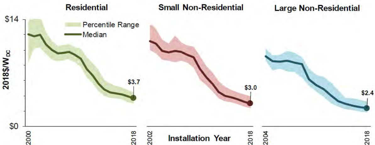
Figure 6-4: Installed price trends ($/W DC ) for residential and commercial PV systems (Source: LBNL [9])
