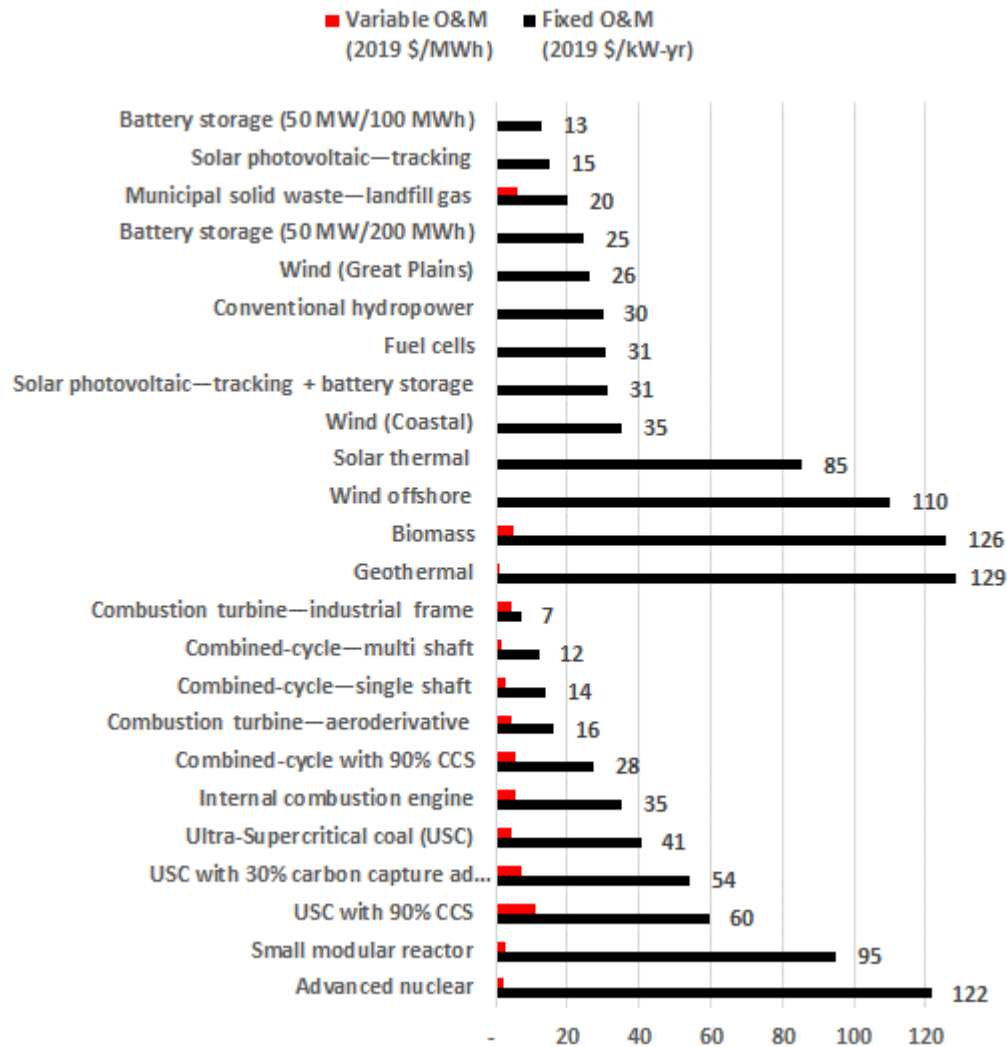
Figure 1-12: Estimated generating technologies fixed and variable O&M cost (Data source: EIA [15])
