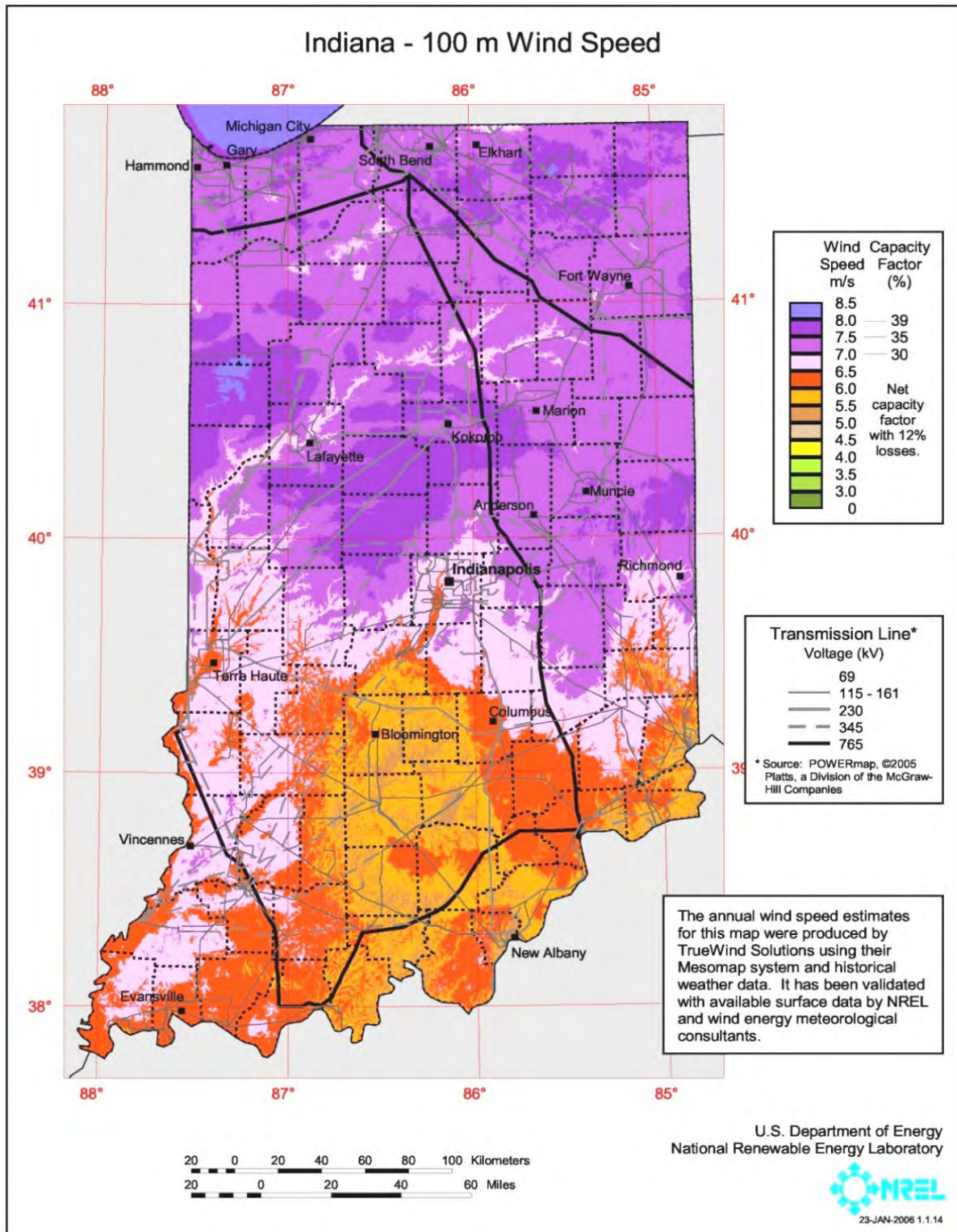
Figure 2-12: Indiana wind speed at 100 meters height (Source: OED/NREL [26])
