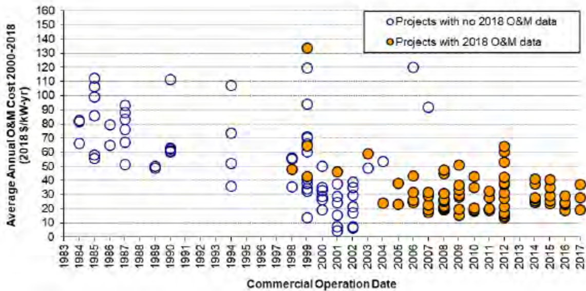
Figure 2-5: Average O&M costs for available data years (Source: LBNL [11])
