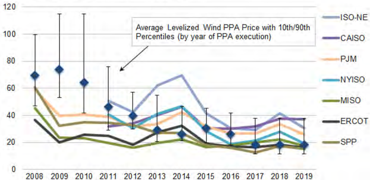
Figure 2-6: Wholesale energy value of wind (Source: LBNL [10])
