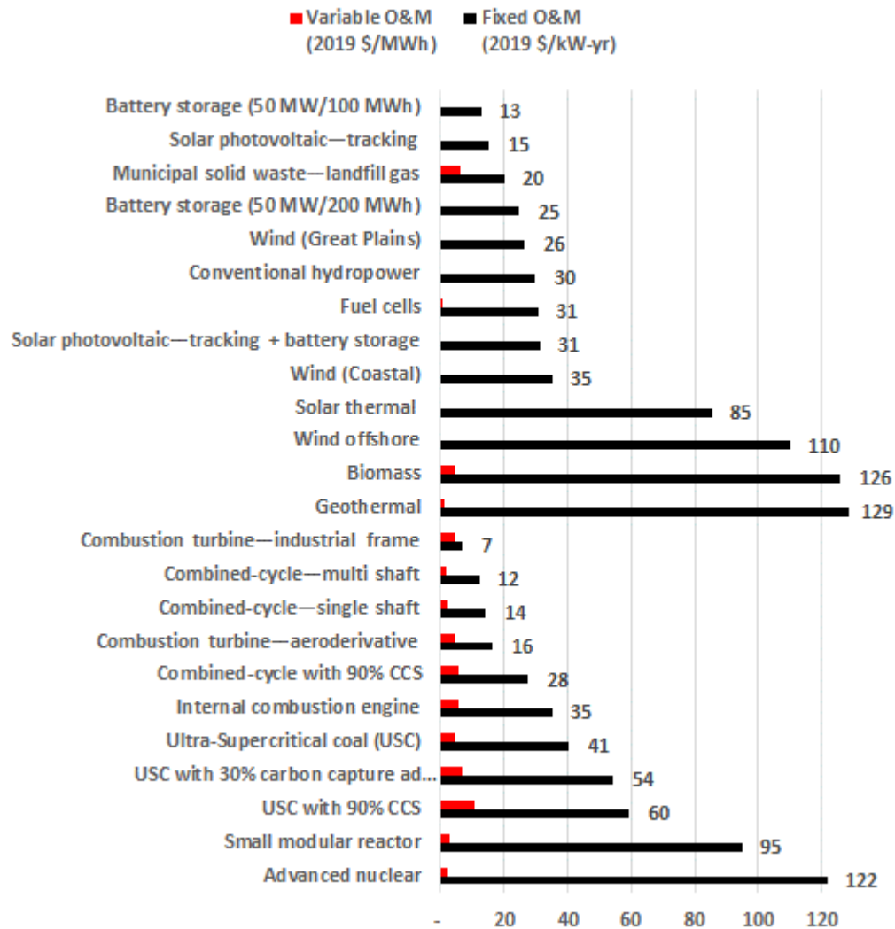
Figure 7-7: Variable and fixed O&M costs of generating technologies (Data source: EIA [13])
