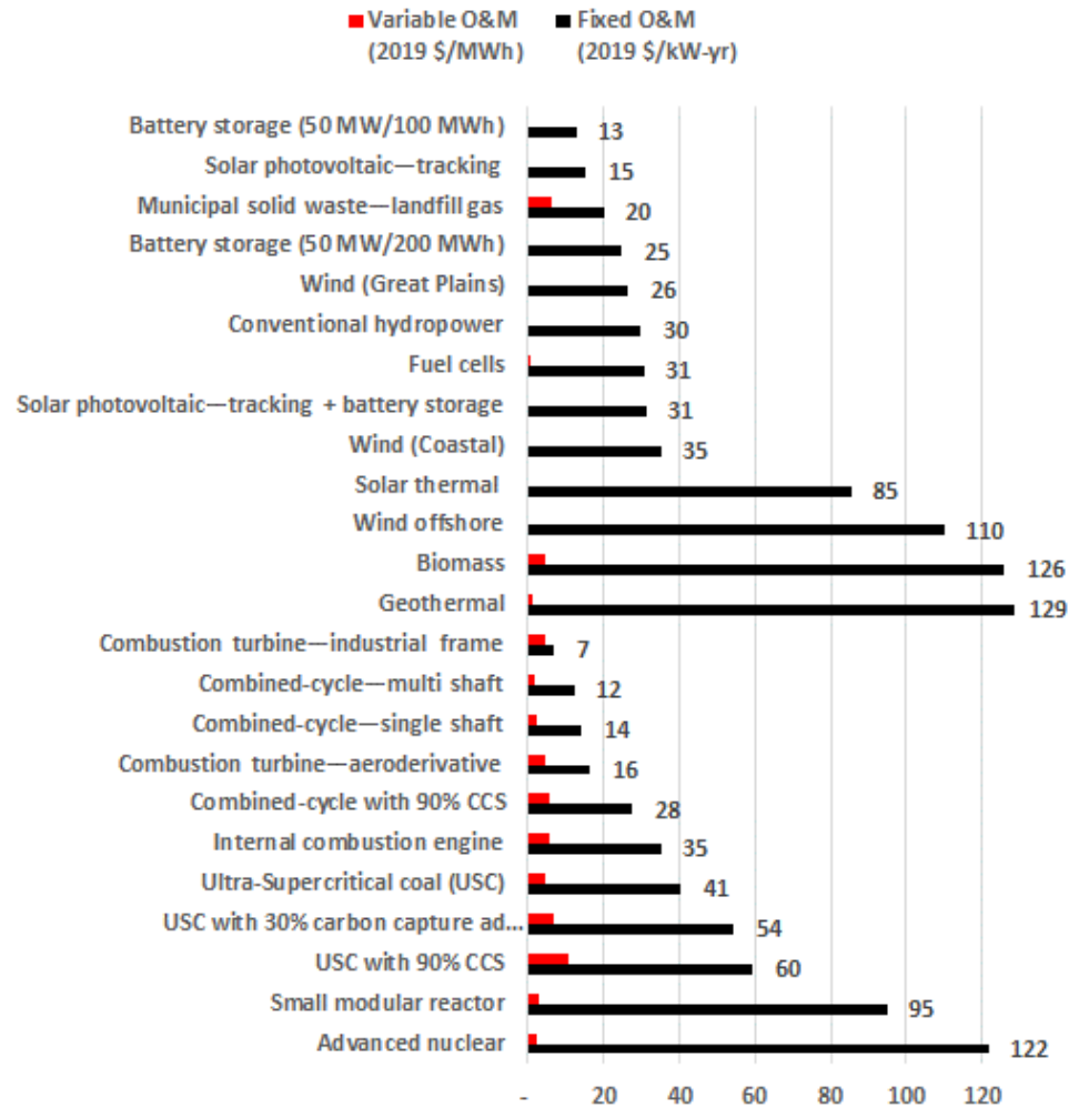
Figure 5-7: Operating and maintenance cost of generating technologies (Data source: EIA [6])
