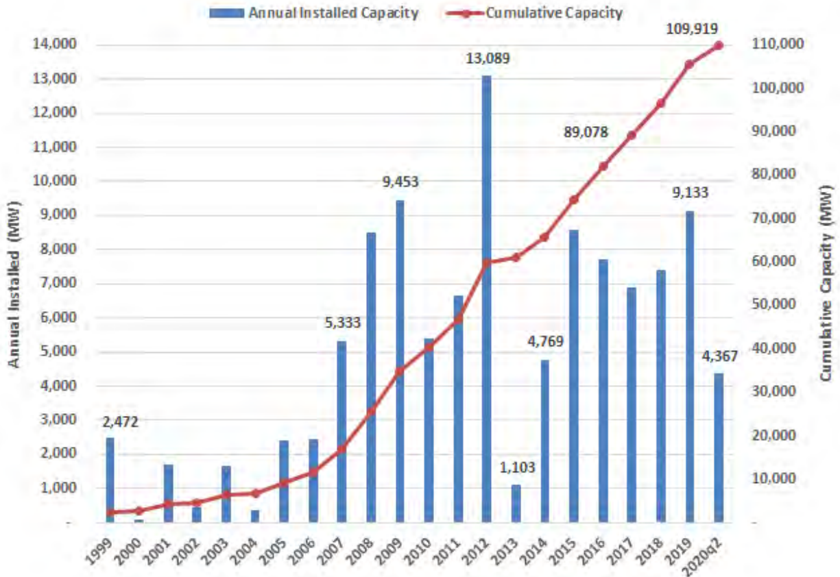
Figure 2-7: U.S. wind capacity growth (Sources: DOE [12], AWEA [13])
