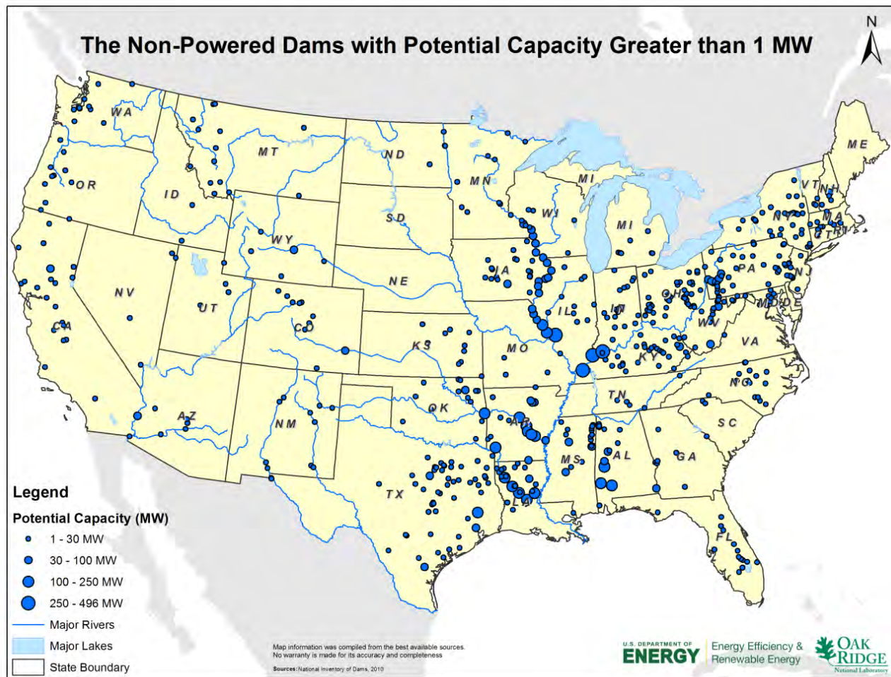
Figure 7-5: Non-powered dams with potential capacity over 1 MW (Source: DOE [19])
