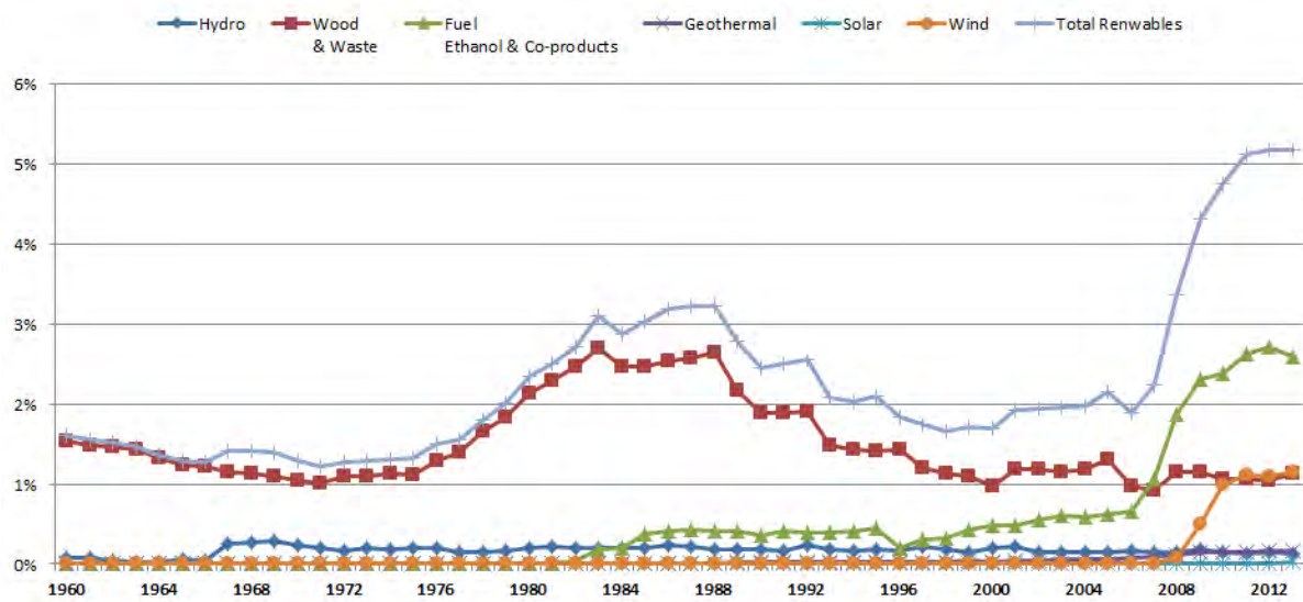
Figure 1-5: Renewables share of Indiana total energy consumption (1960-2013) (Data source: EIA [5])
