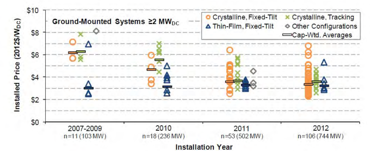
Figure 6-7: Installed price trends over time for utility-scale PV systems (Source: Berkeley [8])
