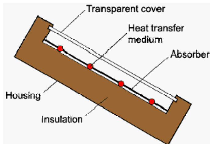
Figure 5-1: Cross-section layout of a flat-plate collector (Source: SolarServer [2])
