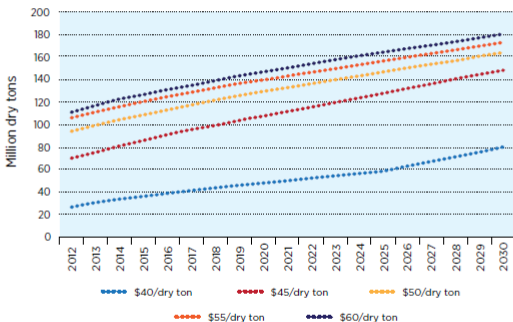
Figure 4-1: Supply of crop residues at various prices under DOE base-case assumptions (Source: DOE [8])
