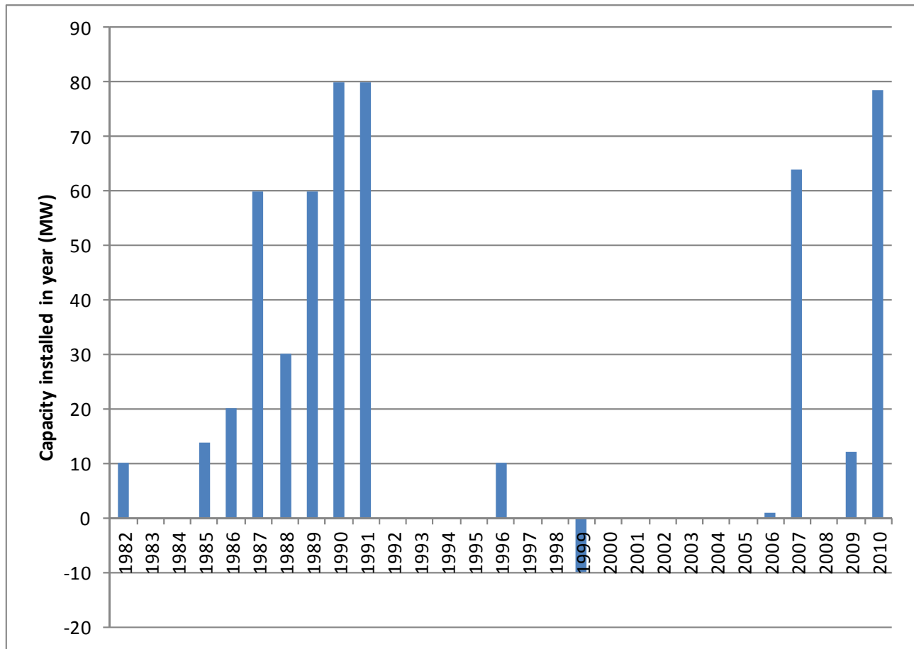
Figure 5-10: U.S. annual net CSP capacity installation (Data source SEIA [10], GoSolar California [11])
