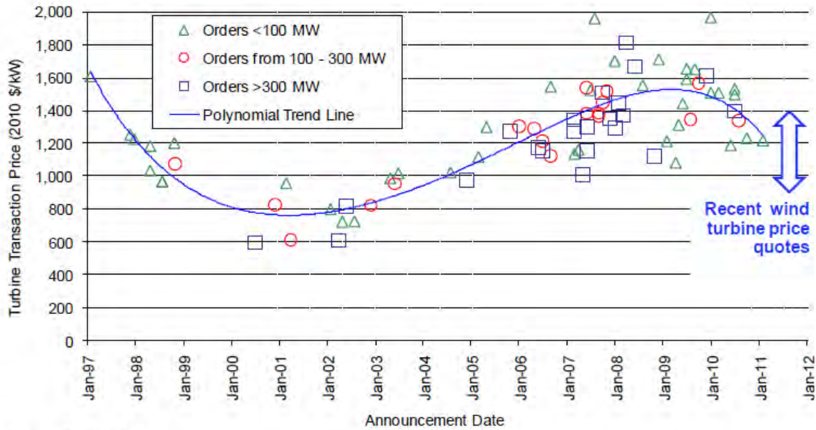
Figure 2-3: Reported U.S. wind turbine prices over time (Source: EERE [7])
