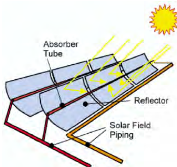
Figure 5-2: A parabolic trough CSP system (Source: NREL [3])
