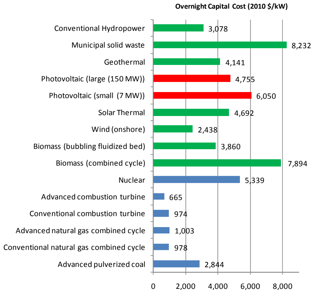
Figure 6-5: Capital cost of generating technologies (Data source: EIA [7])
