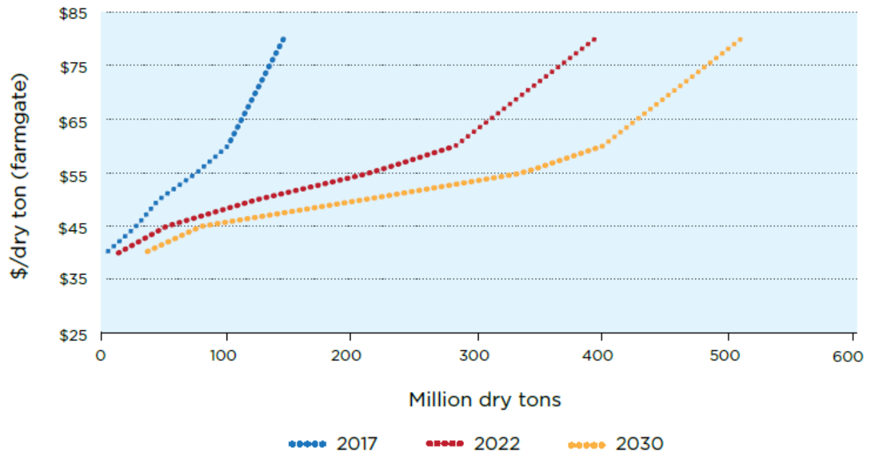
Figure 3-3: Supply curves for all energy crops at selected years (Source: DOE [2])
