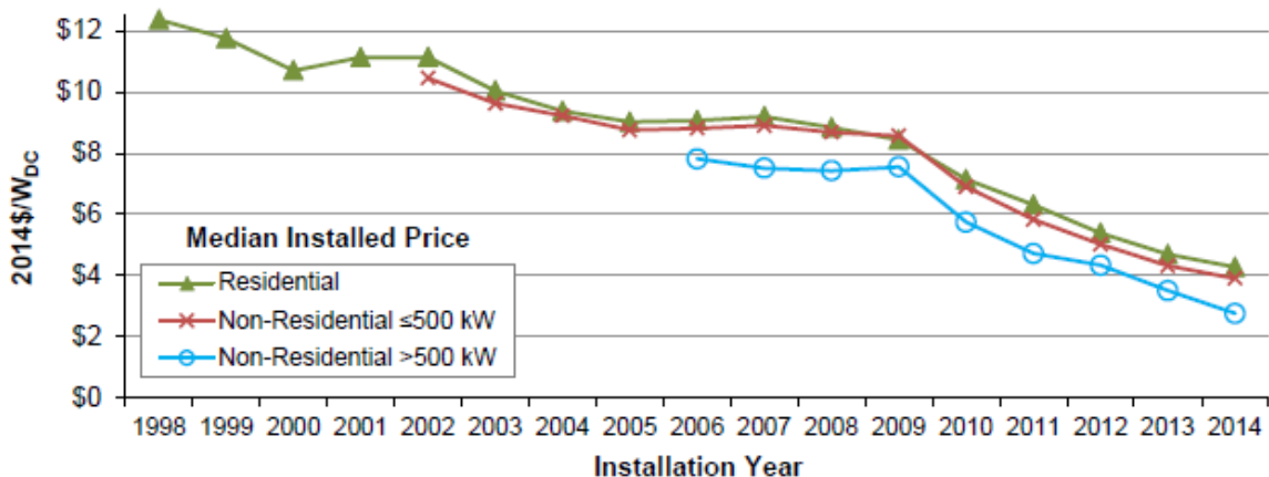
Figure 6-5: Installed price ( \$/W_{DC} 9 ) trends for residential and commercial PV systems (Source: Berkeley National Lab. [10])
