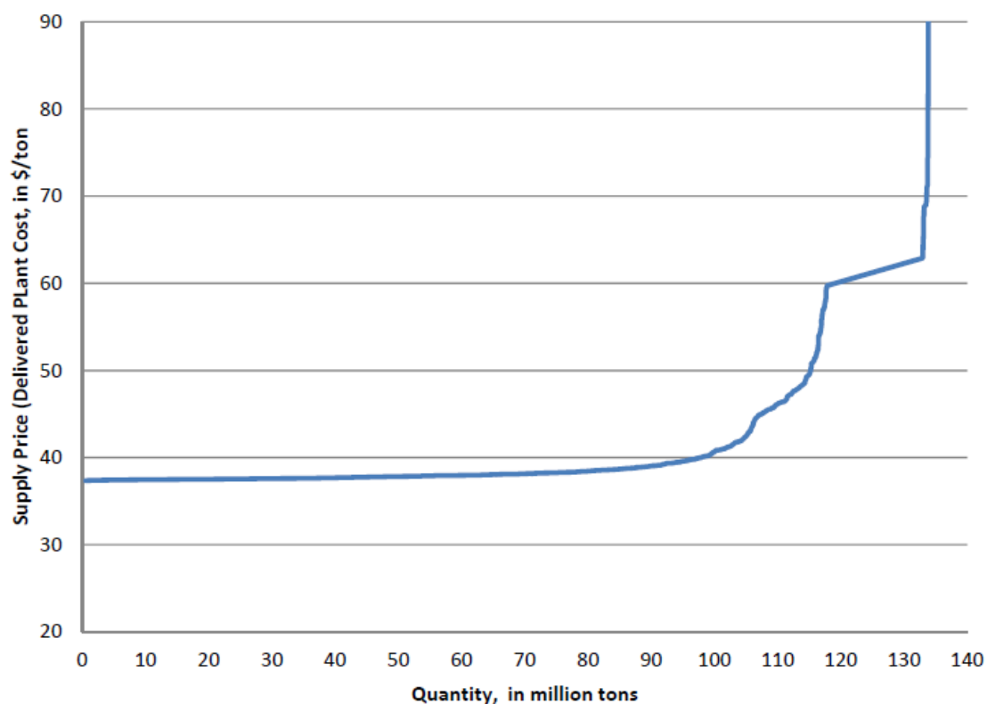
Figure 4-3: U.S. corn stover supply curve (Source: USDA [9])
