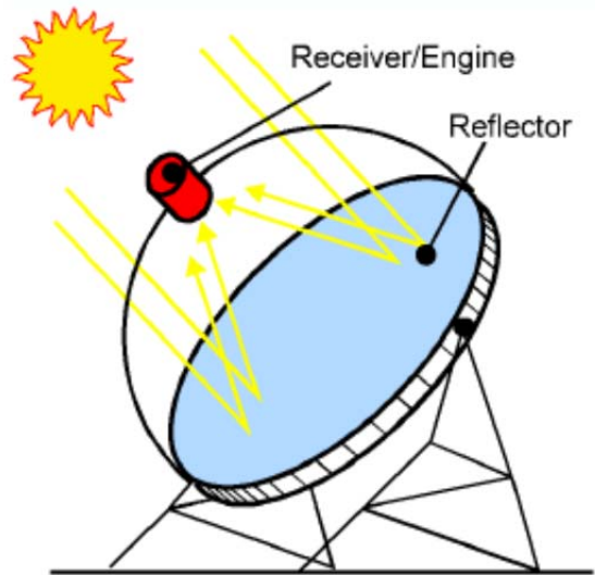
Figure 5-5: A dish/engine CSP system (Source: NREL [2, 3])
