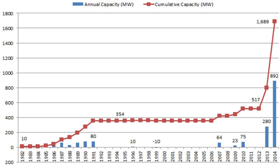
Figure 5-9: Solar thermal power capacity installed in the U.S. (Sources: NREL [4], SEIA [9], IREC [10], Go Solar [11])
