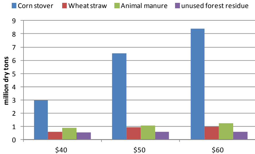
Figure 4-7: Estimated biomass production potential in Indiana (Data source: DOE [8])
