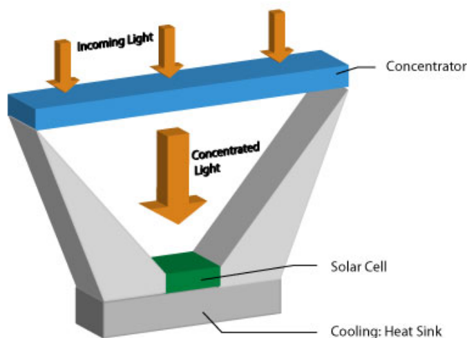
Figure 6-3: Illustration of concentrating photovoltaic cell (Source: Green Rhino Energy [8])
