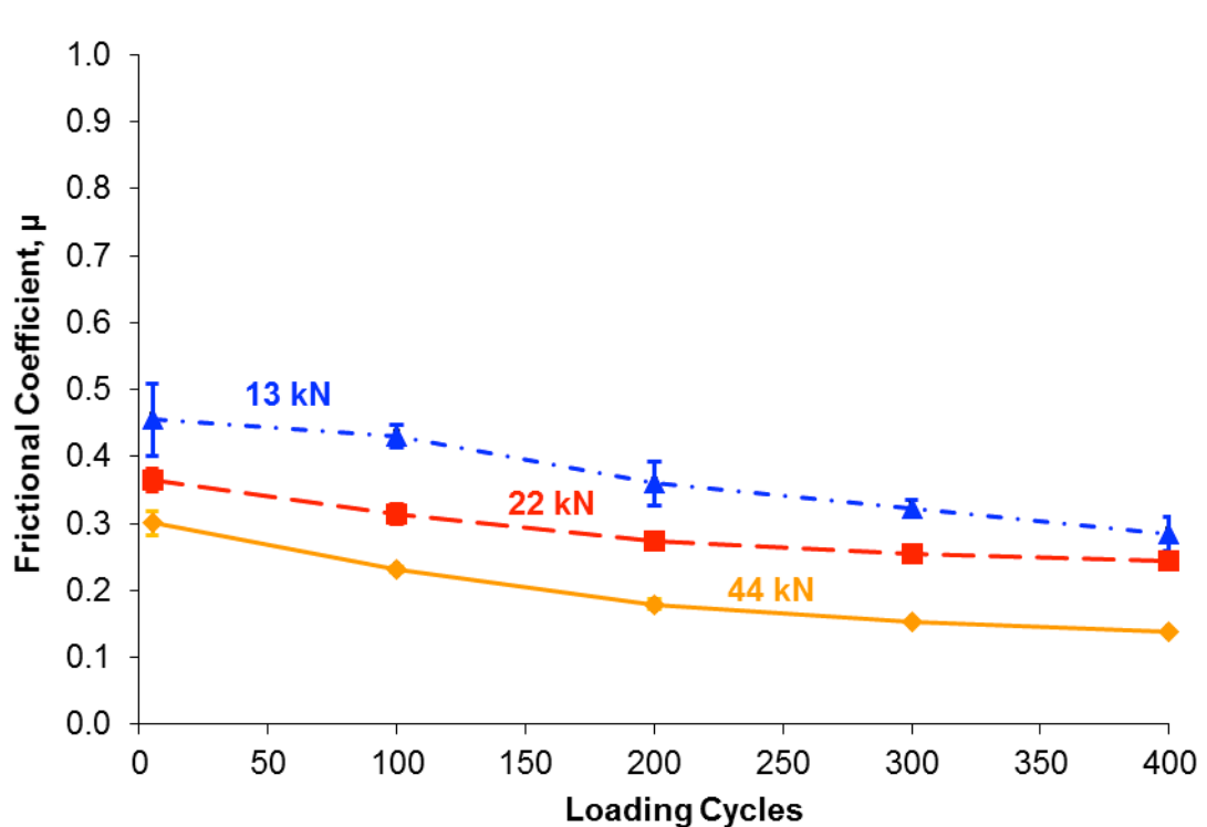
Figure 2.3. Mean COF values of nylon 6/6 pads under 13-kN, 22-kN, and 44-kN normal loads.
