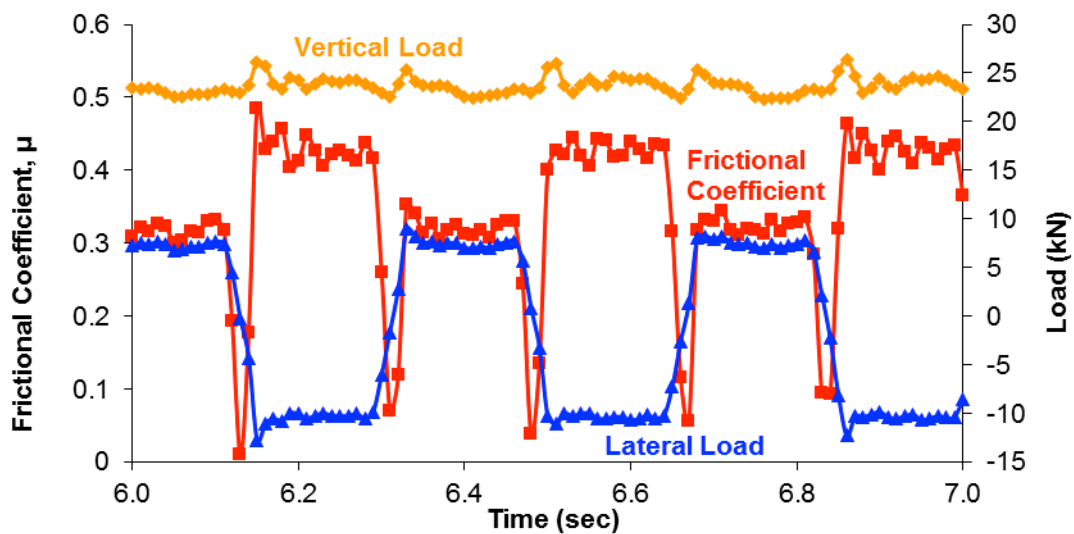
Figure 2.2. Sample frictional coefficient, vertical load, and lateral load during three loading cycles.
