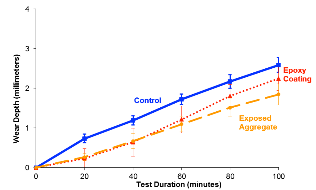
Figure 3.2. Comparison of the average wear depth for each surface treatment.
