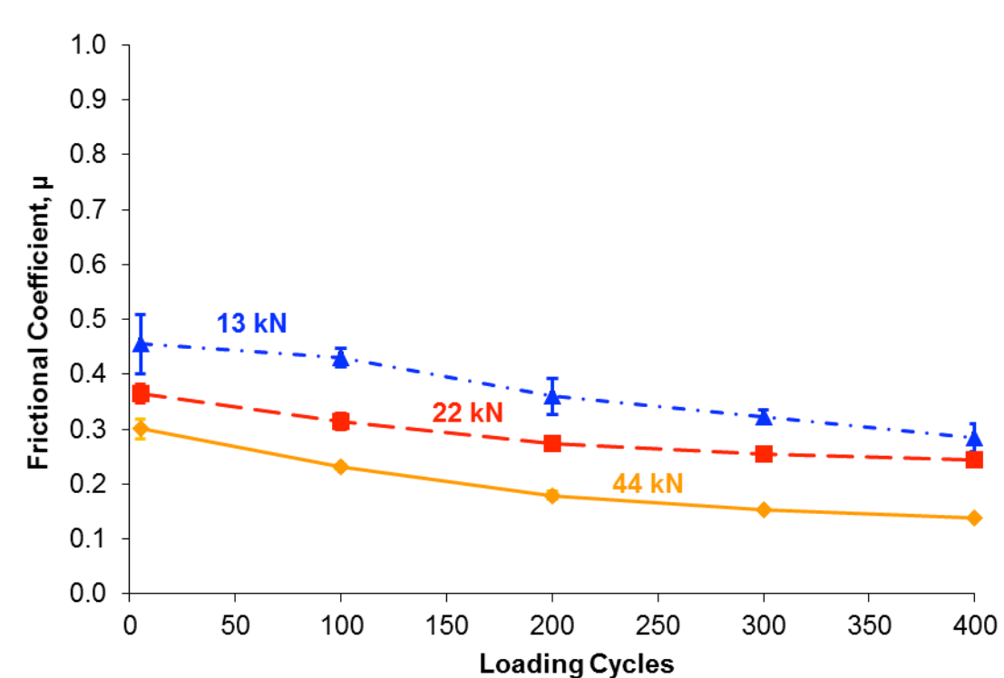
Figure 2.4. Mean COF values of polyurethane pads under 13-kN, 22-kN, and 44-kN normal loads.
