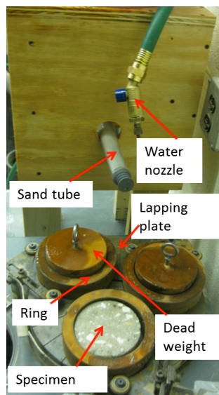
Figure 3.1. SSTAR Test Setup.
