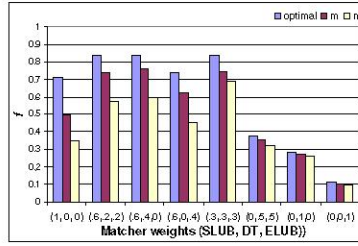
Fig. 3 Effect of combining matchers (BO query logs)
