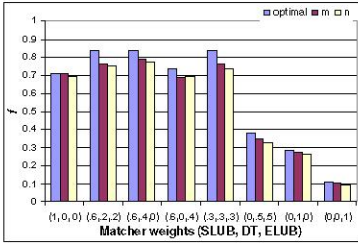
Fig. 2 Effect of combining matchers (BB query logs)
