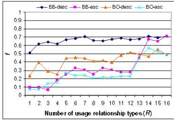
Fig. 5 Effect of usage relationship types
