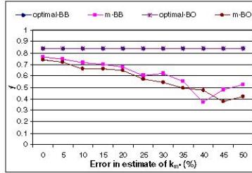
Fig. 6 Effect of varying \hat{k}_{\text{err}}
