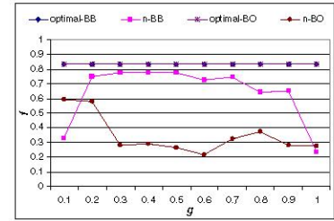
Fig. 7 Effect of varying g
