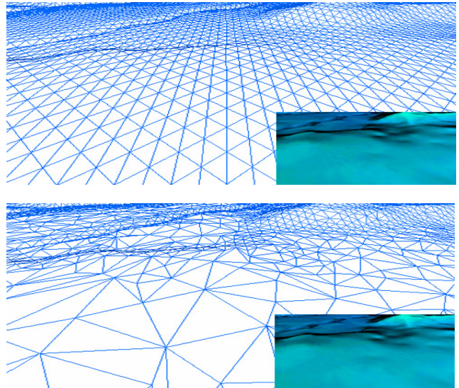
Figure 9. Above: Original TIN generated from a DEM with samples every 10 meters. Insert shows rendered appearance of the original TIN. Below: Simplified TIN and insert showing rendered appearance of simplified TIN. Notice that not only does the simplified TIN appear visually consistent with the original model, but it is also guaranteed to be within a confidence level of the real-world terrain.
