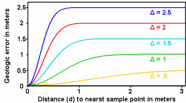
Figure 4. Results of using f(\Delta) = \Delta^2 for the Gaussian distribution in Equation 3.4. Larger values for geologic variation ( \Delta ) provide a sharper rise in error as distance from sample points increase as well as a higher maximum error bound when approaching zero confidence in the linearly interpolated surface.
