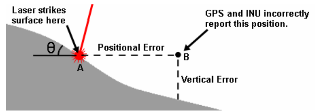
Figure 1. As the slope ( \theta ) of the terrain increases, the error in reported positions from the GPS and INU systems has an increasing effect on the accuracy of vertical measurements.
