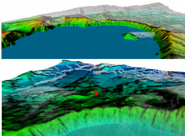
Figure 10. Voxels found to be invisible from the eye-points (shown in red) are displayed as a transparent fog over textured TINs simplified as described in section 5.1. Displaying invisible regions as volumes instead of areas permits the qualification of hiding for units of substantial height.
