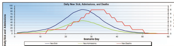
Figure 5: This figure shows our model of patients who have become ill, need hospitalization, or have died from the pandemic. Note the lag in deaths from time of infection as specified by the user.
