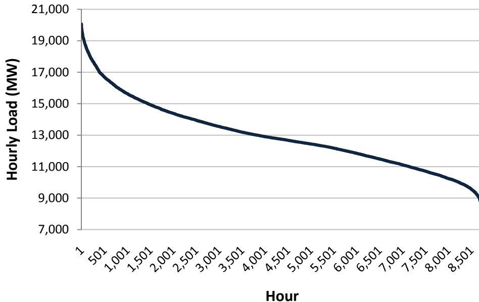
Figure 2. Load duration curve for 2005 Indiana load
