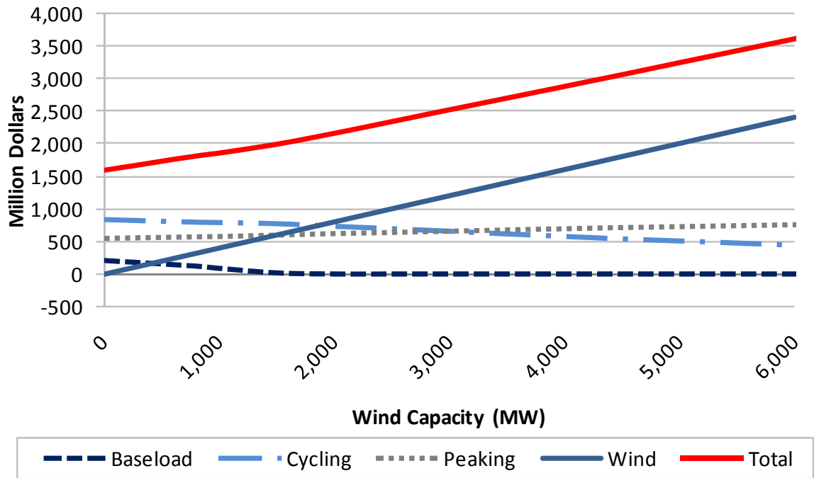
Figure 19. Change in capital costs (relative to base case capacity levels)
