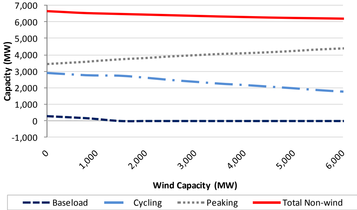
Figure 13. Change in capacity requirements (relative to base case capacity levels)
